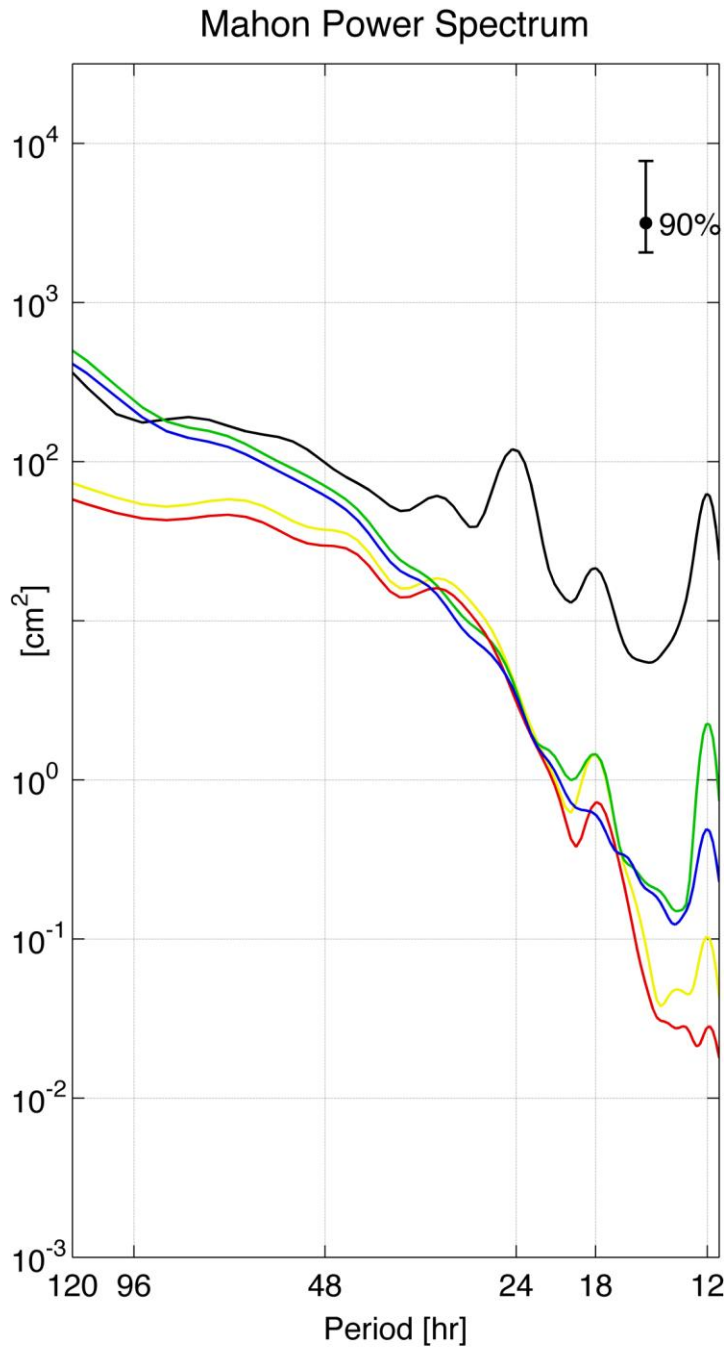
Figure 9 Mahon \eta power spectra from observations and model results. Observations, black; NEMO-MFS1, red; NEMO-MFS2, blue; NEMO-MFS3, yellow; NEMO-MFS4, green.
