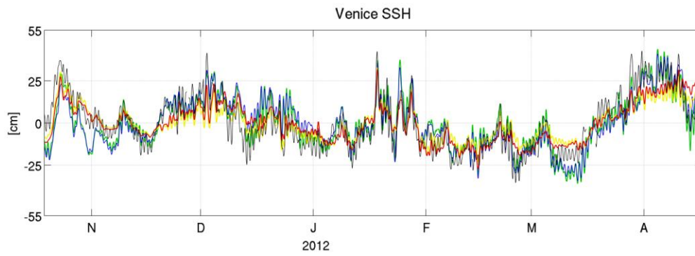
Figure 10 Venice \eta time-series from observations and model results. Data and model results have been filtered with 5 hr running mean. Observations, black; NEMO-MFS1, red; NEMO-MFS2, blue; NEMO-MFS3, yellow; NEMO-MFS4, green.
