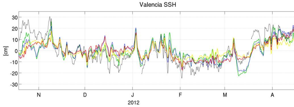
Figure 6 Valencia \eta time-series from observations and models results. Data and model results have been filtered with 5 hr running mean. Observations, black; NEMO-MFS1, red; NEMO-MFS2, blue; NEMO-MFS3, yellow; NEMO-MFS4, green.
