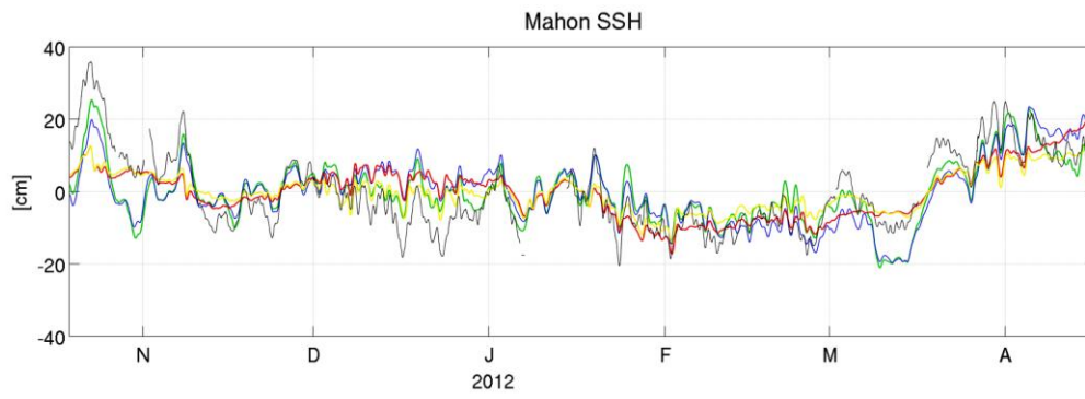
Figure 8 Mahon \eta time-series from observations and model results. Data and model results have been filtered with 5 hr running mean. Observations, black; NEMO-MFS1, red; NEMO-MFS2, blue; NEMO-MFS3, yellow; NEMO-MFS4, green.
