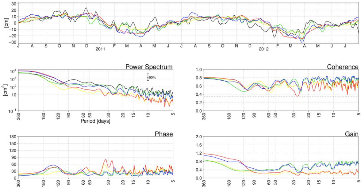
Figure 3 Top Panel: Mediterranean mean sea level time-series from the four experiments and observations averaged over the tide gauge positions shown in Fig. 1. The black line represents observational data, the red line represents NEMO-MFS-1 results, the blue line represents NEMO-MFS-2 results, the yellow line represents NEMO-MFS-3 results, and the green line represents NEMO-MFS-4 results. Left Middle Panel: \eta power spectra for observations and model results, units are cm 2 . Right middle, left bottom and right bottom panels: coherence, phase (degrees) and gain computed between observations and model, respectively. Units in the x axis are periods in days.
