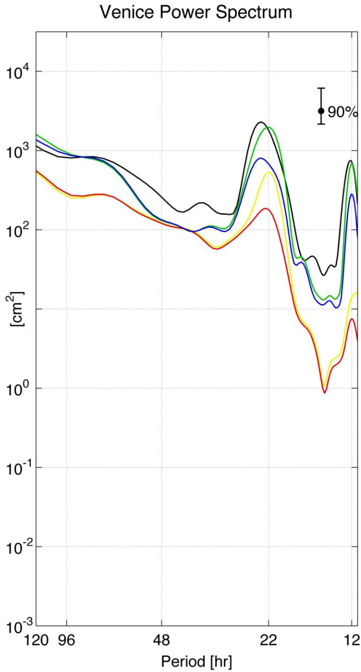
Figure 11 Venice \eta power spectra from observations and model results. Observations, black; NEMO-MFS1, red; NEMO-MFS2, blue; NEMO-MFS3, yellow; NEMO-MFS4, green.
