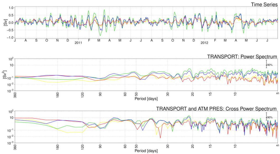
Figure 4 ( Top Panel ) Gibraltar transport time-series from the four experiments. Middle Panels Gibraltar transport power spectra.. Bottom Panels Cross power spectrum between Gibraltar transport and atmospheric pressure. NEMO-MFS1, red; NEMO-MFS2, blue; NEMO-MFS3, yellow; NEMO-MFS4, green.
