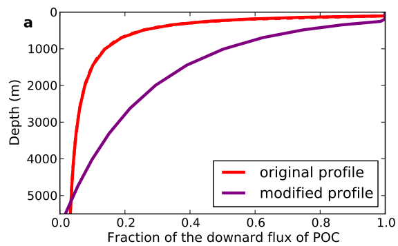
Fig. 2. Fraction of Particulate Organic Carbon (POC) which is transported downward at each level (the fraction not transported is remineralized).
