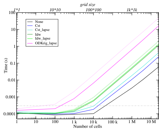
Figure 11. Benchmarks of some spatial interpolation algorithms for various grid sizes for seven input stations (plain lines) and fourteen input stations (dotted lines).
