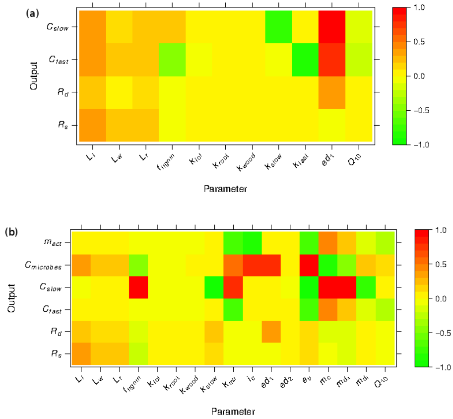
Fig. 2. Sensitivity of the two model to their respective parameters. Outputs tested were all three soil carbon pools including C_{\text{fast}} and C_{\text{slow}} for (a) the chemical model and fast ( C_{\text{fast}} , \text{g C m}^{-2} ), slow ( C_{\text{slow}} , \text{g C m}^{-2} ) and microbial pool ( C_{\text{microbes}} , \text{g C m}^{-2} ) for (b) the biological model. Also the sensitivity of three respiration fluxes were tested including total soil respiration ( R_s , \text{g C m}^{-2} \text{d}^{-1} ), litter respiration ( R_l , \text{g C m}^{-2} \text{d}^{-1} ) and respiration from soil decomposition ( R_d , \text{g C m}^{-2} \text{d}^{-1} ) for both models. Model sensitivity was calculated using the method by Xenakis et al. (2008). Values close or greater to -1 and 1 show high negative and positive sensitivity respectively. For all symbols explanation see Table 1.
