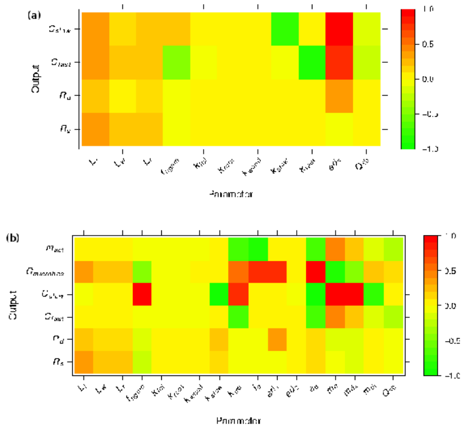
Fig. 2. Sensitivity of the two model to their respective parameters. Outputs tested were all three soil carbon pools including C_{fast} and C_{slow} for a) the chemical model and fast ( C_{fast} , \text{gC m}^{-2} ), slow ( C_{slow} , \text{gC m}^{-2} ) and microbial pool ( C_{microbes} , \text{gC m}^{-2} ) for b) the biological model. Also the sensitivity of three respiration fluxes were tested including total soil respiration ( R_s , \text{gC m}^{-2} \text{d}^{-1} ), litter respiration ( R_l , \text{gC m}^{-2} \text{d}^{-1} ) and respiration from soil decomposition ( R_d , \text{gC m}^{-2} \text{d}^{-1} ) for both models. Model sensitivity was calculated using the method by Xenakis et al. (2008). Values close or greater to -1 and 1 show high negative and positive sensitivity respectively. For all symbols explanation see Table 1.
