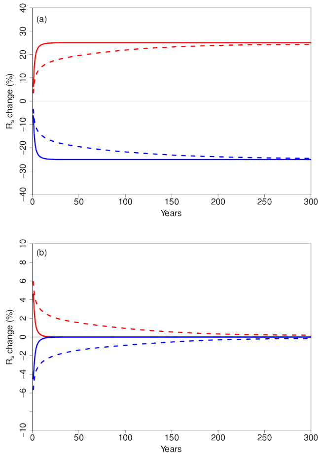
Fig. 4. The percentage change (%) of total soil respiration between the nominal and increased litter (red lines) and the nominal and decreased litter (blue lines) for a) the litter quantity manipulation experiment and b) the temperature manipulation experiment. Solid lines are for the biological and dashed lines for the chemical model. Only the first 300 years of the simulation are shown.
