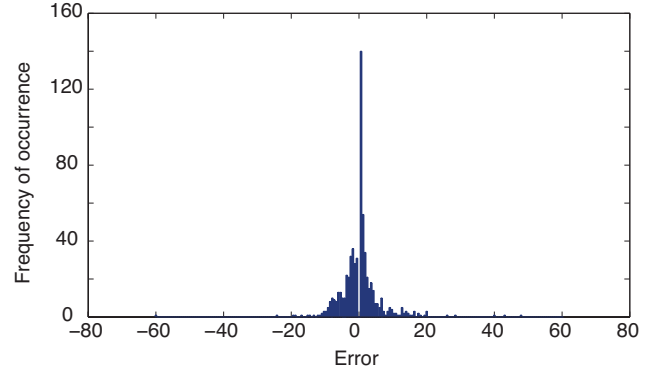
Figure 1. Histogram of the additive error e . For clarity, the zero-error bin has been omitted here.
