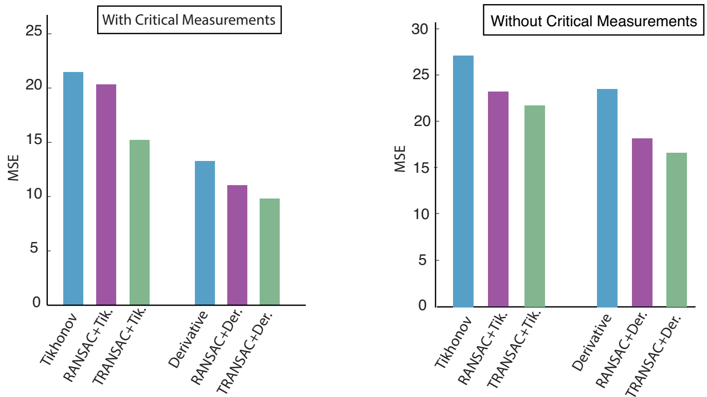
Figure 9. MSE of source estimated by different algorithms. The blue bars correspond with the original algorithms (2, 3). The violet bars indicates that RANSAC is used for outlier removal, and the green ones that TRANSAC is used for outlier removal. The plot on the left was generated using the whole ETEX dataset. The plot on the right was generated using the ETEX dataset without critical measurements.
