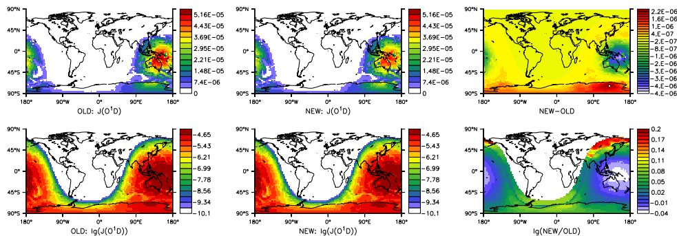
Fig. 2. Comparison of old and new J values (in \text{s}^{-1} ) for \text{O}_3 \rightarrow \text{O}(^1\text{D}) , calculated for 1 January 2000, 02:00 UTC at the surface. The first row is plotted on a linear scale, the second on a logarithmic scale. The left column shows the old result, the center column the new result, and the right column the differences.
