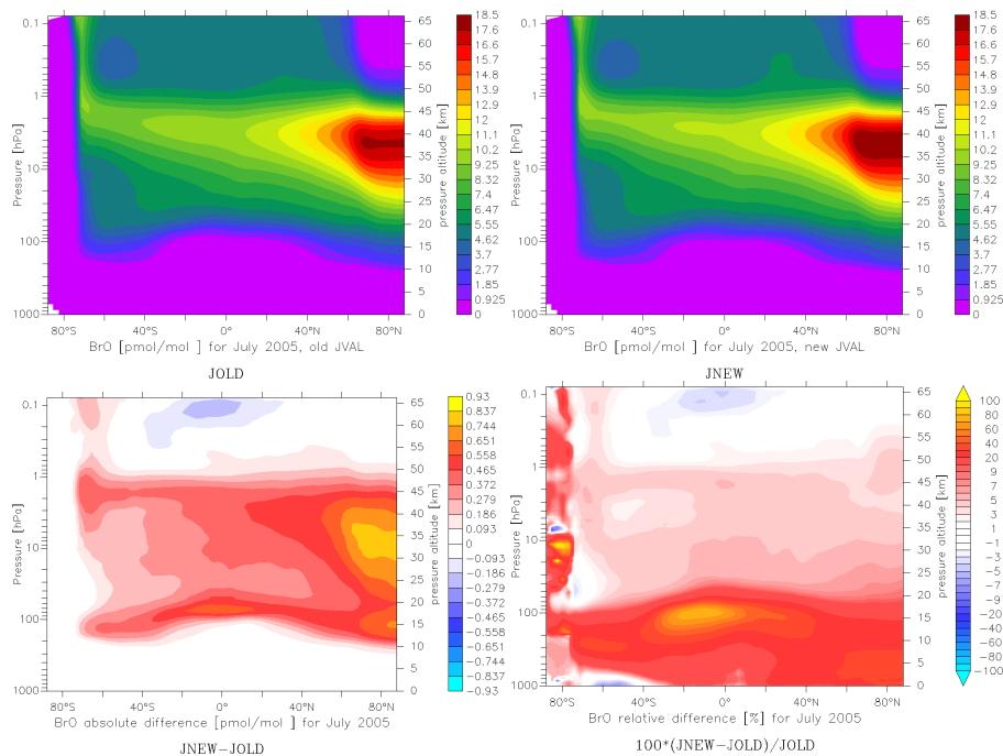
Fig. 5. Effect of updated J values on BrO. All plots refer to monthly mean values of July 2005.
