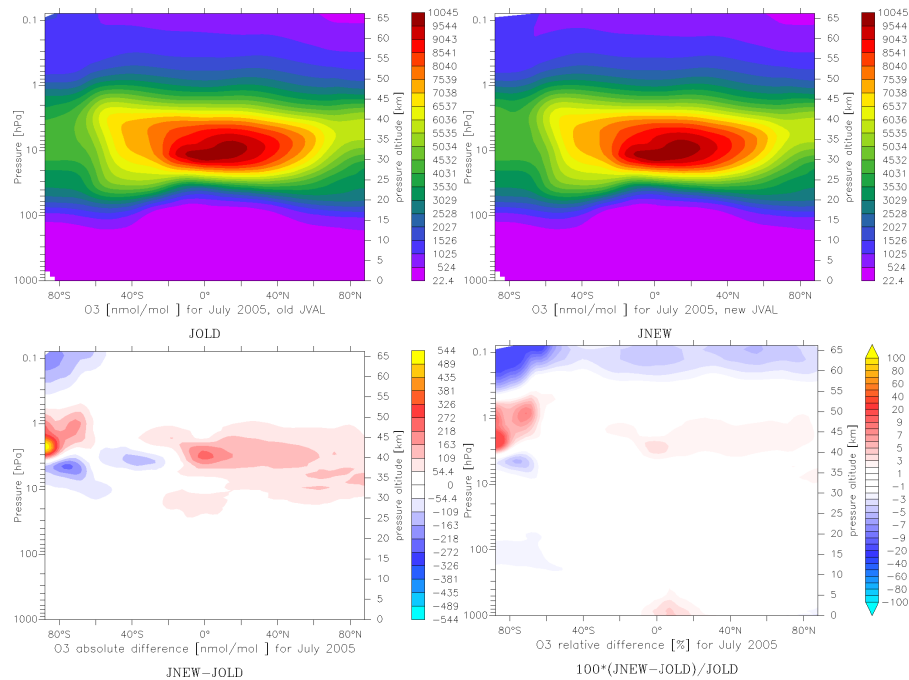
Fig. 4. Effect of updated J values on ozone. All plots refer to monthly mean values of July 2005.
