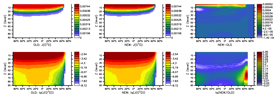
Fig. 3. Comparison of the vertical profiles of the old and new J values (in \text{s}^{-1} ) for \text{O}_3 \rightarrow \text{O}(^1\text{D}) , calculated for 1 January 2000, 02:00 UTC at a longitude of 138^\circ \text{E} and 90 model levels. The first row is plotted on a linear scale, the second on a logarithmic scale. The left column shows the old result, the center column the new result, and the right column the differences.
