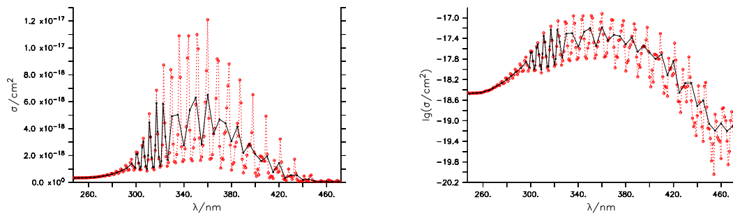
Fig. 1. Absorption cross sections of OCIO on a linear (left) and logarithmic (right) scale. The red line shows the original data taken from S. P. Sander et al. (2011) and the black line after interpolation by JVPP to a fixed grid of 176 wavelengths.
