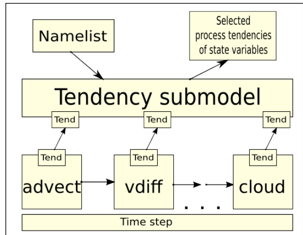
Fig. 2. Schematic of the MESSy TENDENCY submodel within the framework of the EMAC model system. The addition of the individual process tendencies to the total tendency is now outsourced from the respective submodels to the TENDENCY submodel. A user-controlled namelist provides several possibilities for the output of the process tendencies of state variables.
