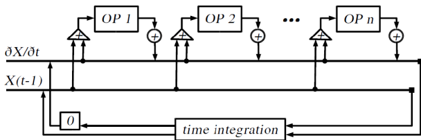
Fig. 1. Operator splitting concept (image taken from Jöckel et al., 2005). For explanation see text. figure
