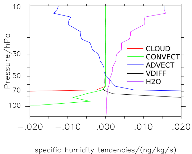
Fig. 10. Zonally averaged process tendencies of the specific humidity (in \text{ng kg}^{-1} \text{s}^{-1} ) at the equator, averaged over the three year time period.
