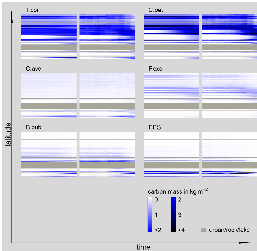
Fig. A9. Carbon mass development of the minor species along the analyzed transect using the stochastic (100 stochastic replicates) LPJ-GUESS approach (right) and the GAPPARD method (left), both with the standard parameter set. Time scale on each plot reaches from 1900 (left side) to 2100 (right side). See Fig. A3 for species abbreviations. Please note that a different color gradient was used than in Fig. A7.
