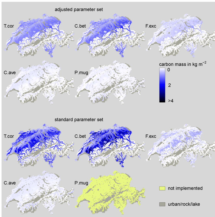
Fig. A5. Carbon mass simulated with the adjusted and standard parameter set for minor species at 2000. C.bet: Carpinus betulus ; C.ave: Coryllus avelanna ; F.exc: Fraxinus excelsior ; P.mug: Pinus mugo ; T.cor: Tilia cordata . Please note that a different color gradient was used than in Fig. A3.
