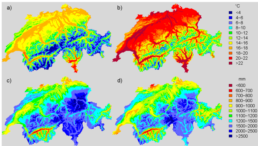
Fig. A2. Development of temperature and precipitation over time under the used SRES A1B scenario. (a) Mean summer temperature (June, July, August) for the 1900–1930 period; (b) mean summer temperature for the 2070–2100 period; (c) mean annual precipitation for the 1900–1930 period; (d) mean annual precipitation for the 2070–2100 period.
