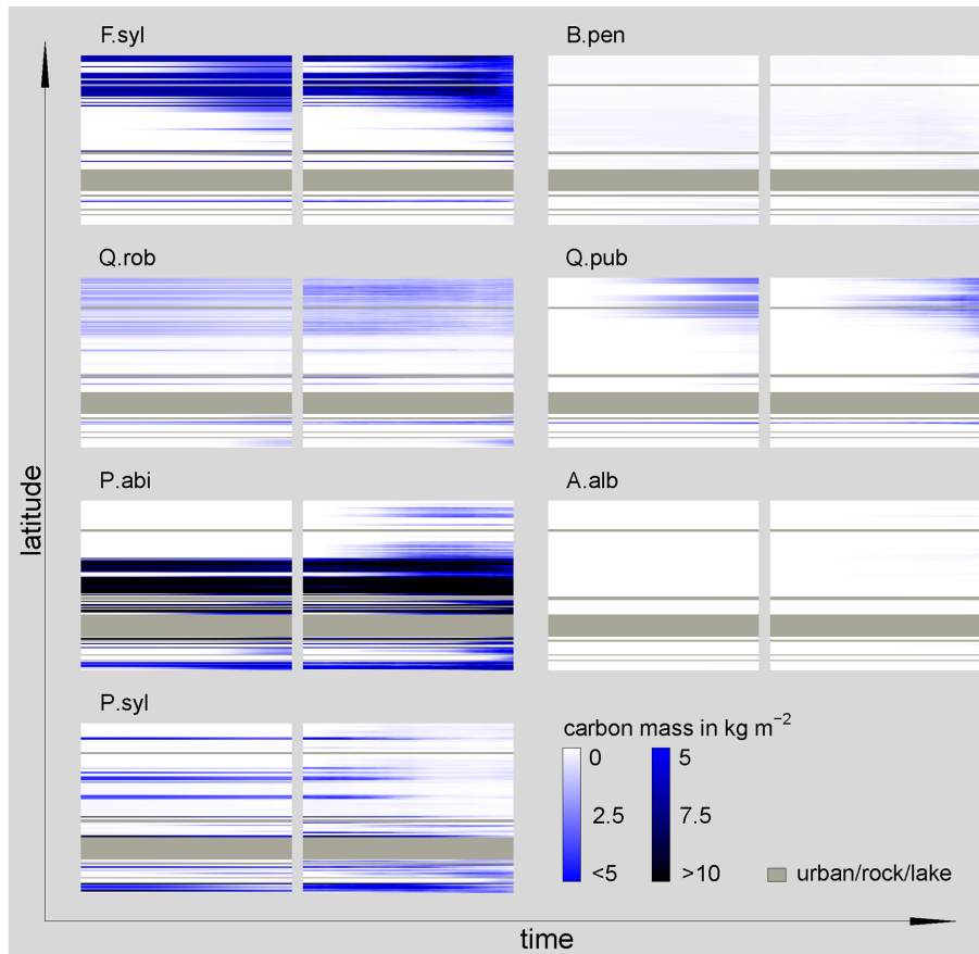
Fig. A7. Carbon mass development along the analyzed transect of seven selected species using the stochastic (100 stochastic replicates) LPJ-GUESS approach (right) and the GAPPARD method (left), both with the standard parameter set. Time scale on each plot reaches from 1900 (left side) to 2100 (right side). See Fig. A3 for species abbreviations.
