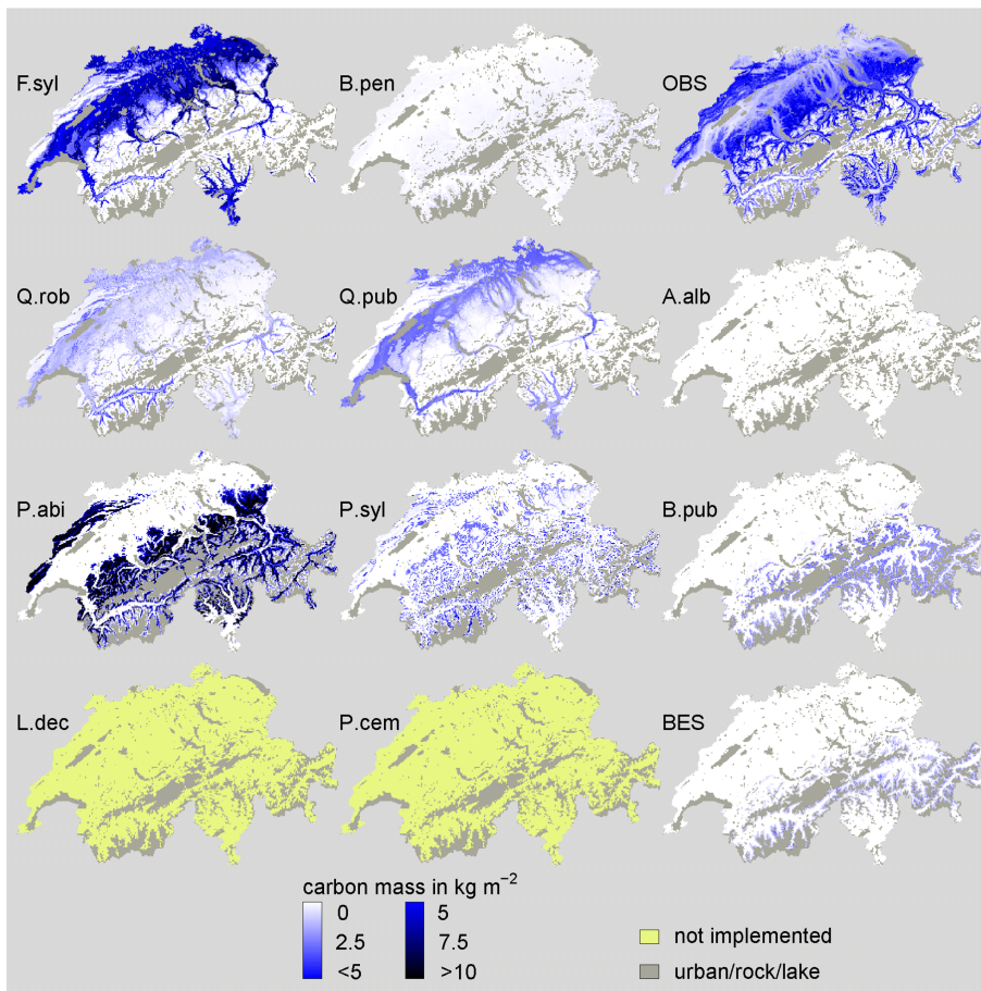
Fig. A4. Carbon mass simulated with the standard parameter set for single species at 2100. See Fig. A3 for species abbreviations.
