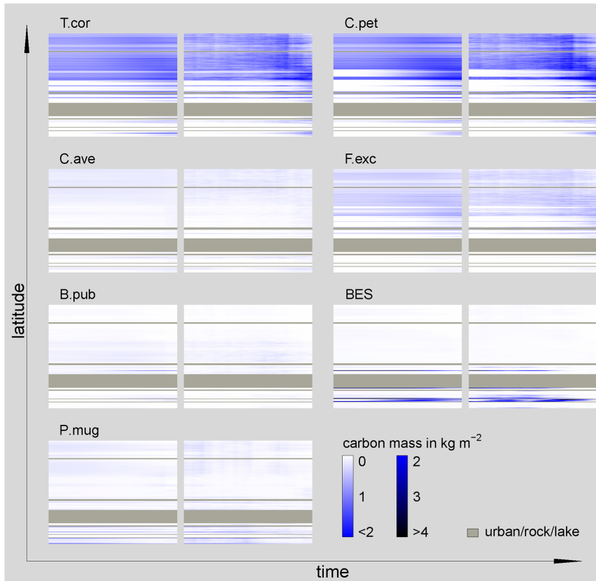
Fig. A8. Carbon mass development of the minor species along the analyzed transect using the stochastic (100 stochastic replicates) LPJ-GUESS approach (right) and the GAPPARD method (left), both with the adjusted parameter set. Time scale on each plot reaches from 1900 (left side) to 2100 (right side). See Fig. A3 for species abbreviations. Please note that a different color gradient was used than in Fig. A7.
