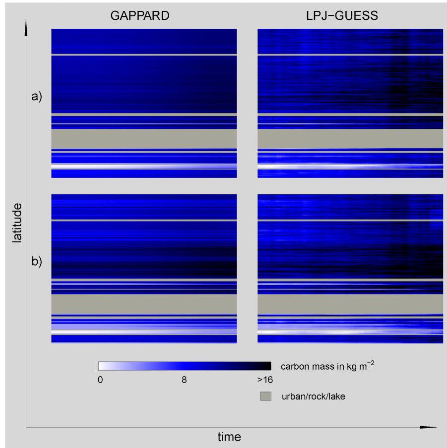
Fig. 2. Total carbon mass development along the analyzed transect from 1900 (left side) to 2100 (right side) with LPJ-GUESS (100 stochastic replicates) and using the GAPPARD method. (a) adjusted parameter set; (b) standard parameter set.
