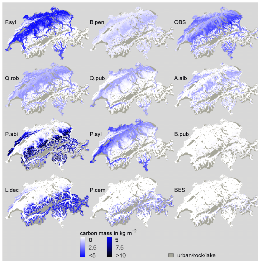
Fig. A3. Carbon mass simulated with the adjusted parameter set for single species at 2100. A.alb: Abies alba ; B.pen: Betula pendula ; B. pub: Betula pubescens ; F.syl: Fagus sylvatica ; L.dec: Larix decidua ; P.abi: Picea abies ; P.cem: Pinus cembra ; P.syl: Pinus sylvestris ; Q.pub: Quercus pubescens ; Q.rob: Quercus robur ; BES: boreal evergreen shrubs; OBS: other broadleaved species.
