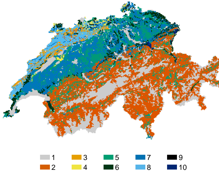
Fig. A1. Soil code used in LPJ-GUESS simulations. 1 – urban, rocky or water areas (no forest growth) 2 – E: 5.0. V: 0.110. D0: 0.2. D15: 0.800. D100: 0.4 3 – E: 4.0. V: 0.115. D0: 0.2. D15: 0.650. D100: 0.4 4 – E: 4.0. V: 0.127. D0: 0.2. D15: 0.650. D100: 0.4 5 – E: 4.5. V: 0.130. D0: 0.2. D15: 0.725. D100: 0.4 6 – E: 4.0. V: 0.150. D0: 0.2. D15: 0.650. D100: 0.4 7 – E: 3.5. V: 0.135. D0: 0.2. D15: 0.575. D100: 0.4 8 – E: 3.0. V: 0.120. D0: 0.2. D15: 0.500. D100: 0.4 9 – E: 0.2. V: 0.100. D0: 0.2. D15: 0.500. D100: 0.4 10 – E: 9.0. V: 0.300. D0: 0.1. D15: 0.100. D100: 0.1 E: empirical parameter in percolation equation ( k_1 ) ( \text{mm day}^{-1} ); V: volumetric water holding capacity at field capacity minus volumetric water holding capacity at wilting point, as fraction of soil layer depth; D0, D15 and D100: thermal diffusivity ( \text{mm}^2 \text{s}^{-1} ) at 0%, 15% and 100% water holding capacity.
