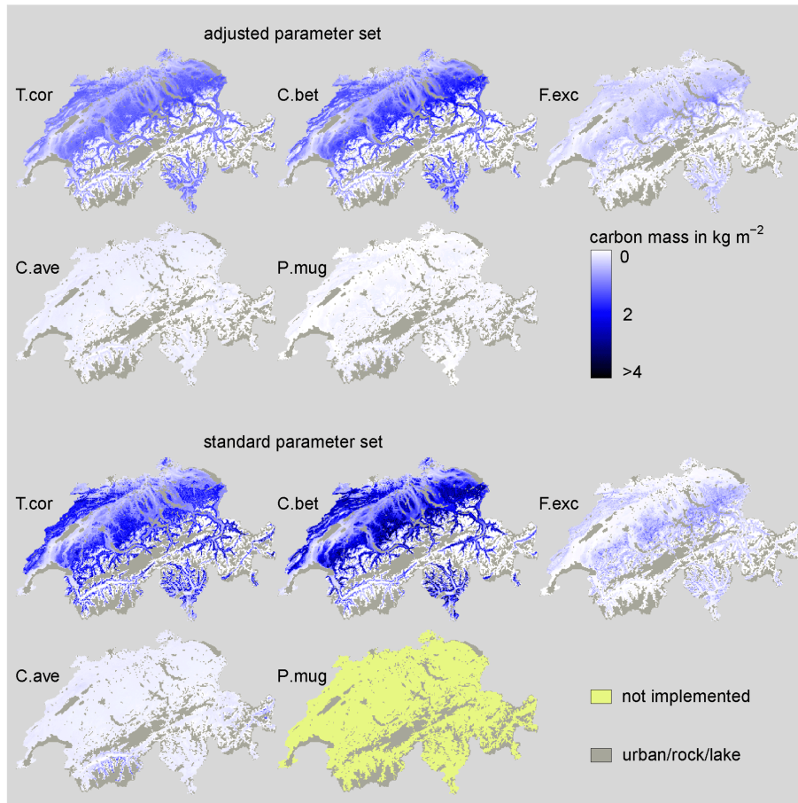
Fig. A6. Carbon mass simulated with the adjusted and standard parameter set for minor species at 2100. See Fig. A5 for species abbreviations. Please note that a different color gradient was used than in Fig. A3.
