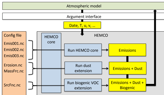
Fig. 3. Use of HEMCO extensions to compute emissions with functional dependencies on local environmental variables. Three standard emission inventories (Emis001.nc - Emis003.nc) and two extensions (dust emissions and biogenic VOC emissions) are combined. The extensions use external gridded data (Erosion.nc, MassFrc.nc, SrcFnc.nc) and compute additional scale factors dependent on temperature (T), wind (u, v), etc., imported from the atmospheric model through the argument interface. All selected HEMCO extension are sequentially called after the HEMCO core module, and the emission arrays calculated therein become added to the emissions previously calculated in HEMCO core. See Section 2.6 for more details.
