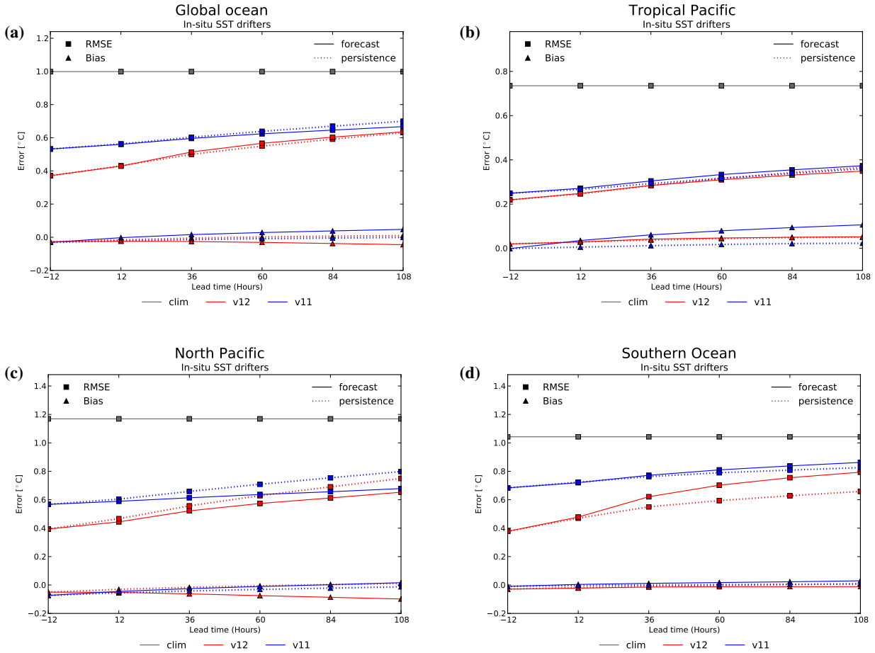
Fig. 6. Forecast lead-time plots showing RMS errors (squares) and mean errors (triangles) against surface temperature measurements (°C) taken by in-situ drifting buoys for the (a) global, (b) Tropical Pacific, (c) North Pacific and (d) Southern Ocean regions. Statistics are shown for model forecasts (solid lines) and persistence (dotted lines) averaged over all forecasts performed during the trials for the v12 (red) and v11 (blue) systems and the EN3 climatology (grey). The x-axis represents forecast lead-time (in hours) ranging from the analysis fields at T-12h up to the 5-day forecasts at T+108h.
