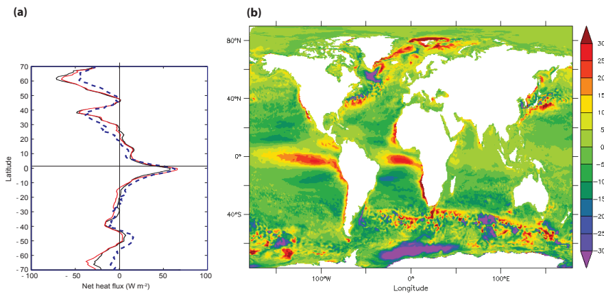
Figure 10. (a) Zonal mean net air-sea heat flux in GO1 (black); GO5.0 (red) and CORE2 data (dashed blue line) in years 1996-2005; and (b) surface net downward heat flux difference GO5.0 minus GO1.
