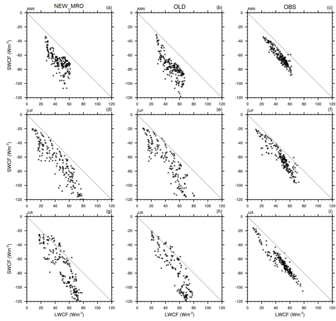
Fig. 1 Scatter diagram of SW CRF vs. LW CRF over the tropical warm pool region ( 10^{\circ} S- 20^{\circ} N, 110^{\circ} E- 160^{\circ} E) for NEW_MRO (left), OLD (central) and CERES_EBAF (right) in ANN (a-c), DJF (d-f) and JJA (g-i).
