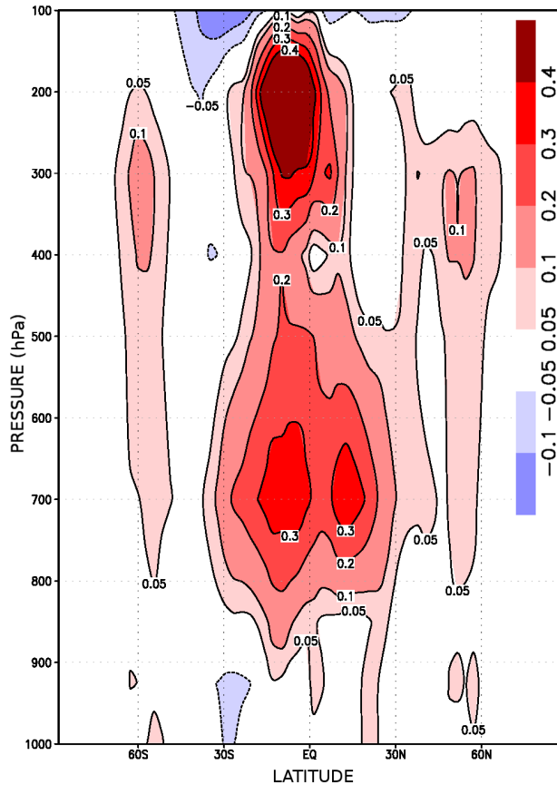
Fig. 9. Pressure-latitude cross section of forecast day three zonal mean energy norm differences (unit \text{J/kg m}^2 \text{ Pa} ) between default and optimized model from January to March 2011. Positive values indicate where the optimized model is performing better.
