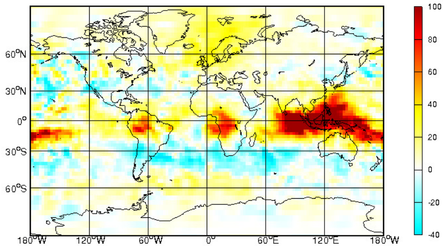
Fig. 7. Forecast day three kinetic energy mean difference (unit \text{J}/\text{kg m}^2 \text{ Pa} ) of the optimized and default model from January to March 2011. Positive values indicate improved day-three forecasts after parameter optimization.
