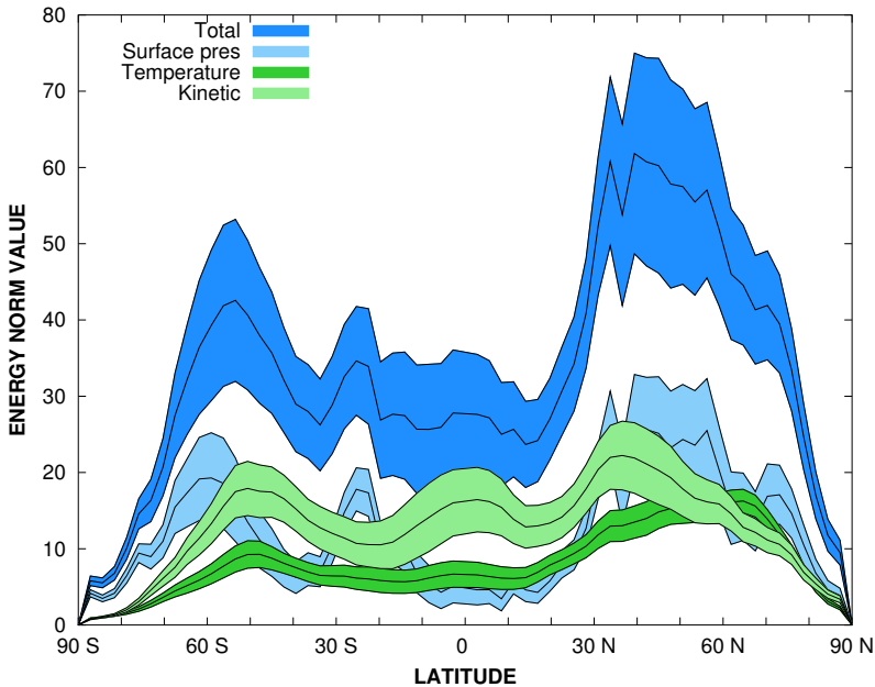
Fig. 1. Mean error and ensemble spread of zonally-averaged and areal-weighted energy norm (unit \text{J}/\text{kg m}^2 \text{ Pa} ) for 15 days (1st to 15th of January 2011) from +72 h forecast. Dry total energy norm (dark blue), and individual terms; surface pressure (light blue), temperature (dark green) and kinetic energy (light green). Continuous black line indicates the mean model error. Width of the colored area represents \pm two standard deviations from the mean.
