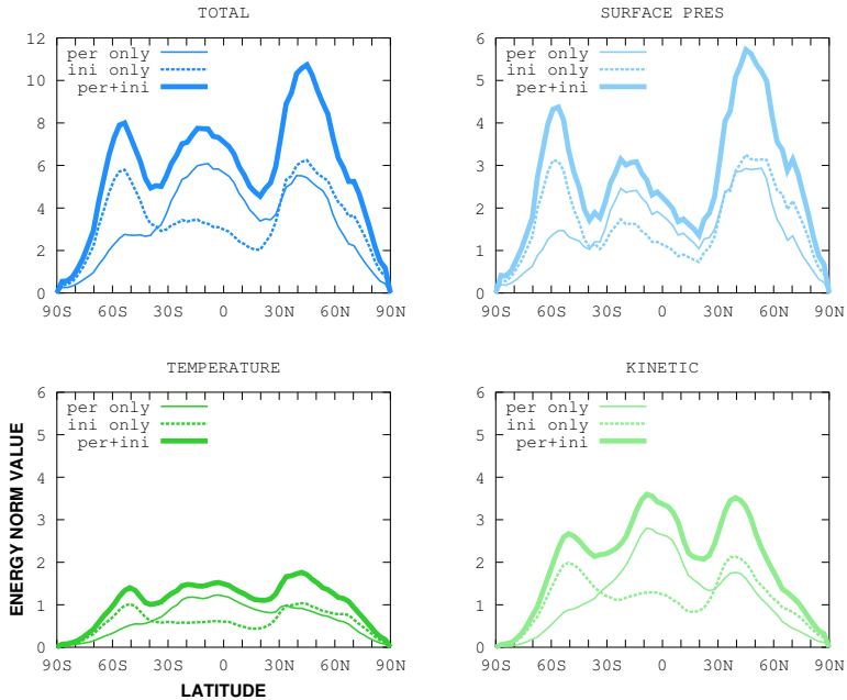
Fig. 2. Ensemble spread (two times standard deviation; unit \text{J/kg m}^2 \text{ Pa} ) at forecast day three averaged over 30 ensembles. Spreads of dry total energy norm (total), and surface pressure (surface pres), temperature and kinetic energy (kinetic) terms. Experiments with only parameter perturbations active (thin continuous lines), only initial state perturbations active (dashed lines), and both sources of uncertainty active (thick continuous line).
