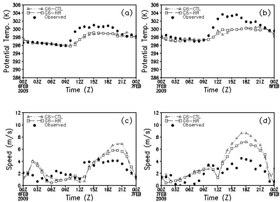
Figure 9: HR and CTL potential temperature and wind speed against observational data from the Jacarepaguá (JPA) station.
