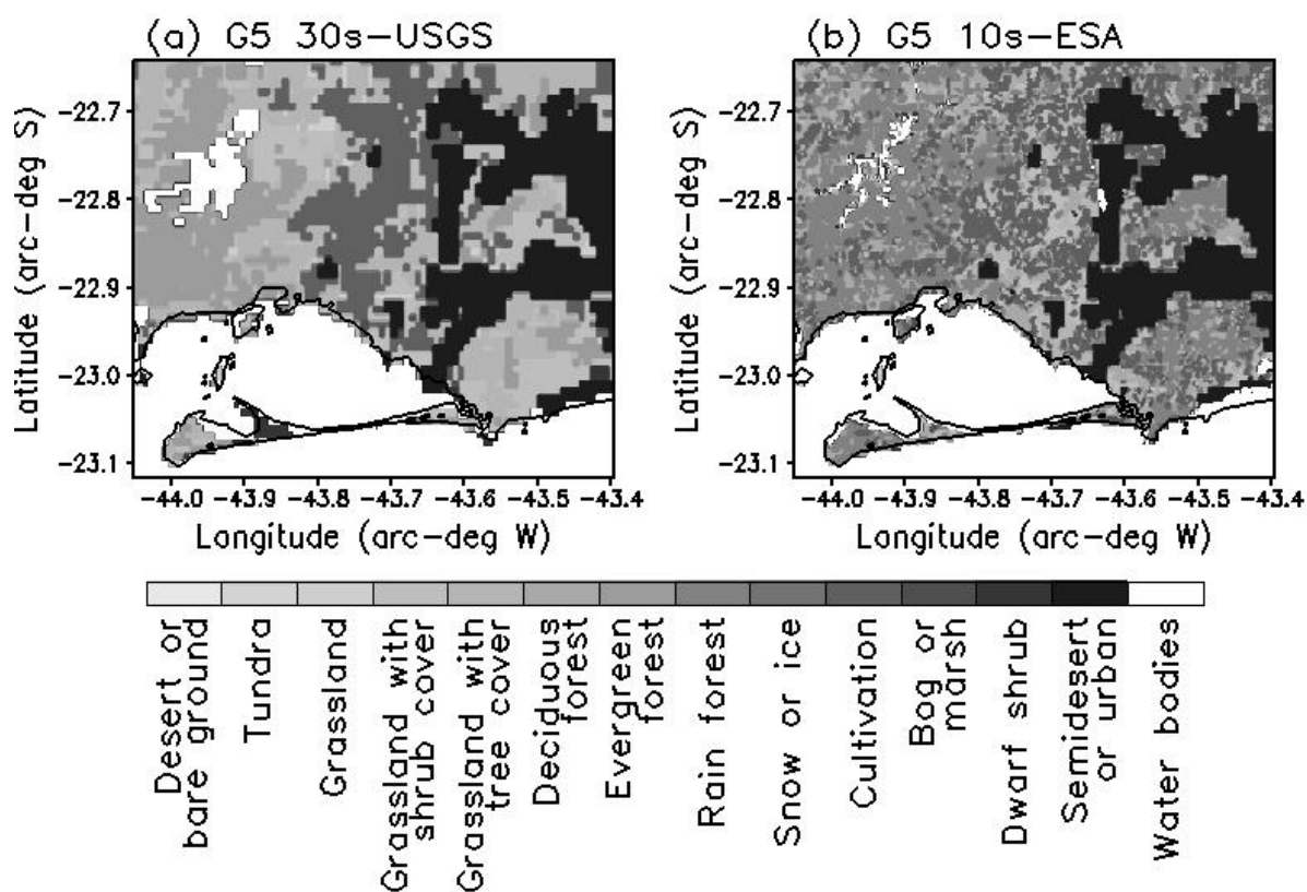
3 Figure 5. Vegetation-type shaded maps for G5, processed with (a) 30s-USGS and (b) 10s- 4 ESA databases.
