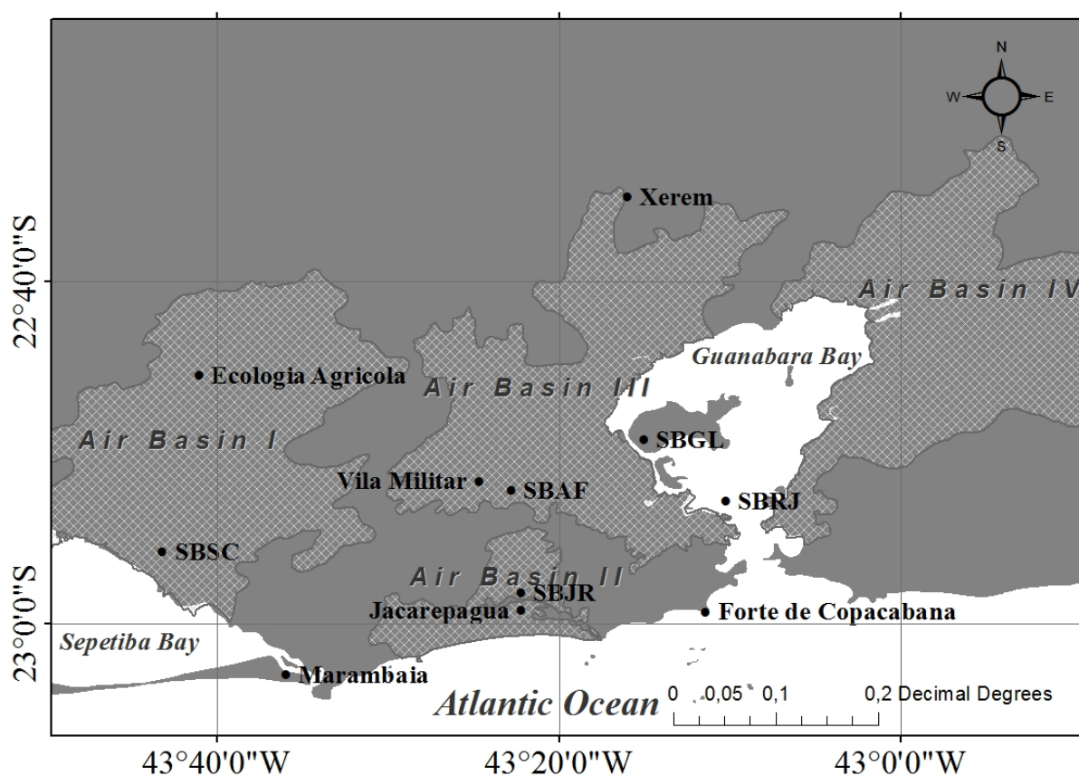
3 Figure 1. The Metropolitan Area of Rio de Janeiro's (MARJ) air basins and the location of the 4 surface weather-observation stations.
