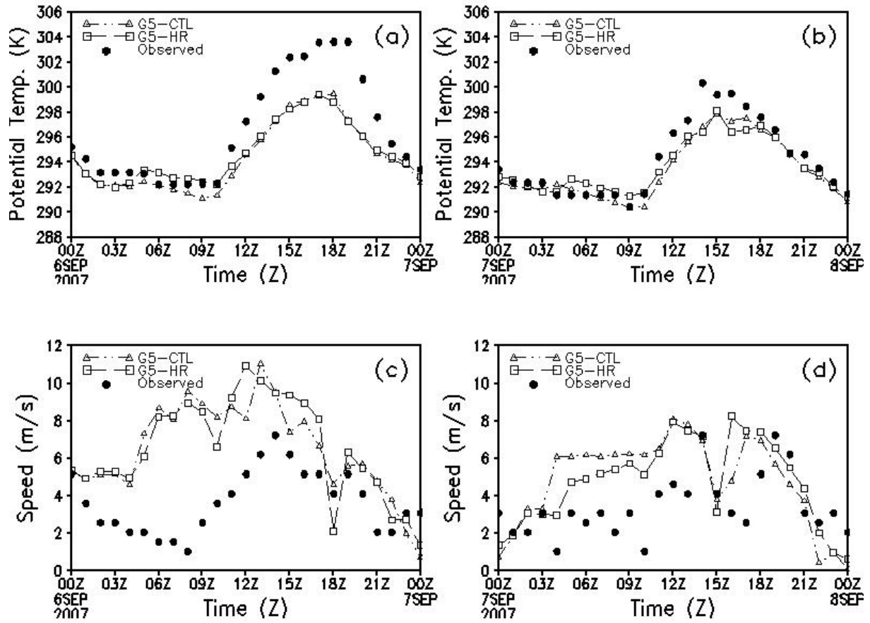
3 Figure 9. Time cross-section data of (a-b) potential temperature \theta (K), and (c-d) wind speed 4 ( \text{m s}^{-1} ) observed (closed circle) and simulated by G5 of CTL (open triangle) and HR (open 5 square) runs for 00:00 UTC 06 September to 00:00 UTC 08 September 2007 at SBSC surface 6 weather-observation station.
