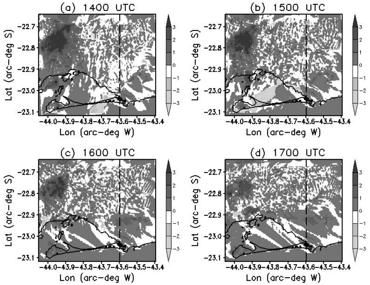
3 Figure 15. Horizontal cross-section of the difference of potential temperature (K - shaded 4 areas) between runs for the G5 domain, calculated as \theta(\text{HR}) - \theta(\text{CTL}) , for (a) 14:00 UTC, (b) 5 15:00 UTC, (c) 16:00 UTC and (d) 17:00 UTC 07 September 2007.
