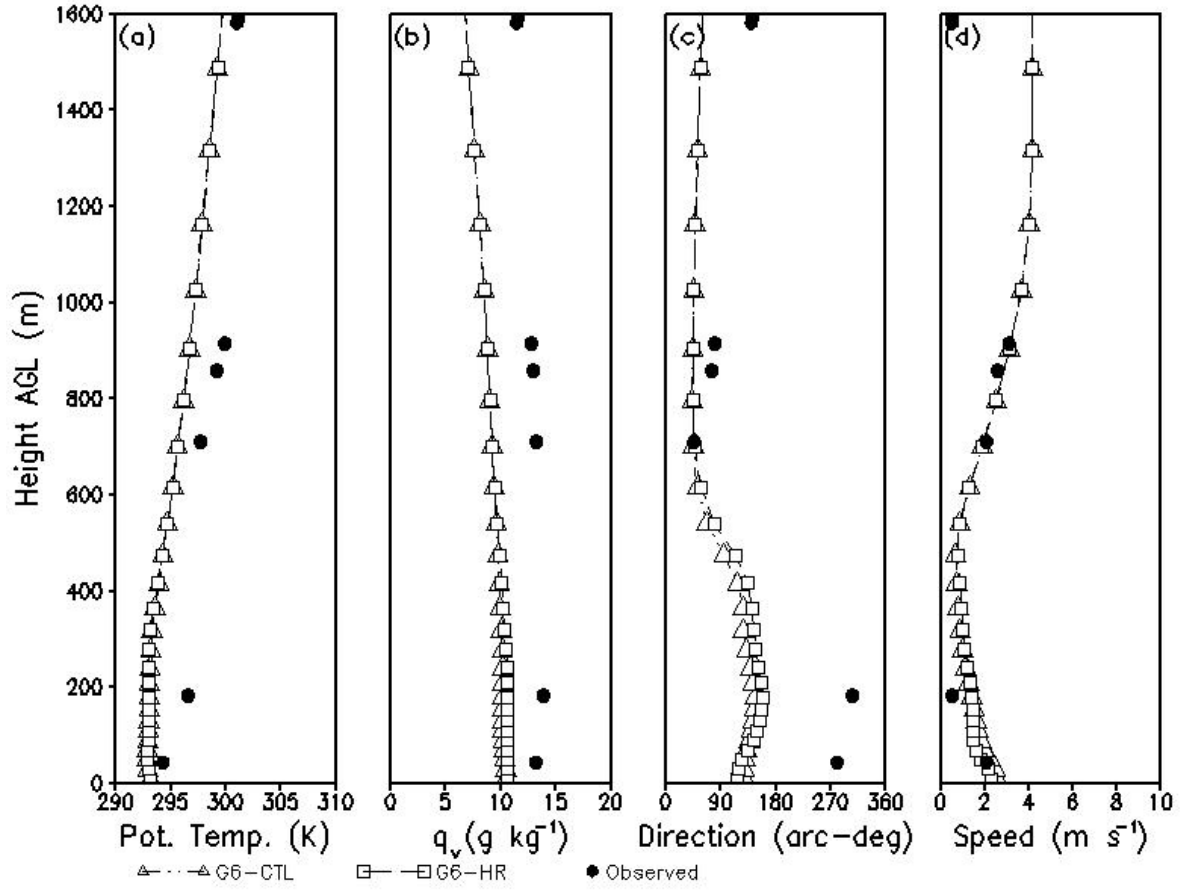
3 Figure 14. Vertical data profiles of (a) potential temperature \theta (K), (b) water-vapor mixing 4 ratio q_v ( \text{g kg}^{-1} ), (c) wind direction (arc-deg) and (d) speed ( \text{m s}^{-1} ) observed (closed circle) and 5 simulated by G6 of CTL (open triangle) and HR (open square) runs for 12:00 UTC 07 6 September 2007 at SBGL upper-air weather station.
