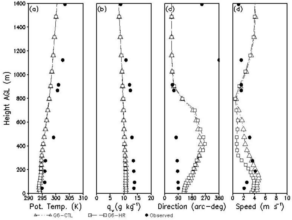
3 Figure 13. Vertical data profiles of (a) potential temperature \theta (K), (b) water-vapor mixing 4 ratio q_v ( \text{g kg}^{-1} ), (c) wind direction (arc-deg) and (d) speed ( \text{m s}^{-1} ) observed (closed circle) and 5 simulated by G6 of CTL (open triangle) and HR (open square) runs for 12:00 UTC 06 6 September 2007 at SBGL upper-air weather-observation station.
