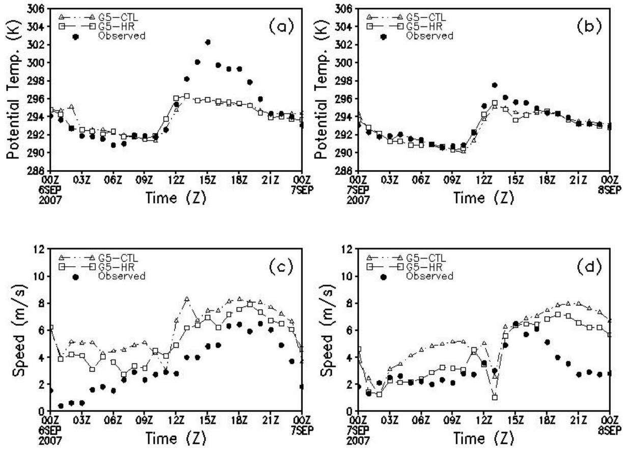
3 Figure 7. Time cross-section data of (a-b) potential temperature \theta (K), and (c-d) wind speed 4 ( \text{m s}^{-1} ) observed (closed circle) and simulated by G5 of CTL (open triangle) and HR (open 5 square) runs for 00:00 UTC 06 September to 00:00 UTC 08 September 2007 at Marambaia 6 surface weather-observation station.
