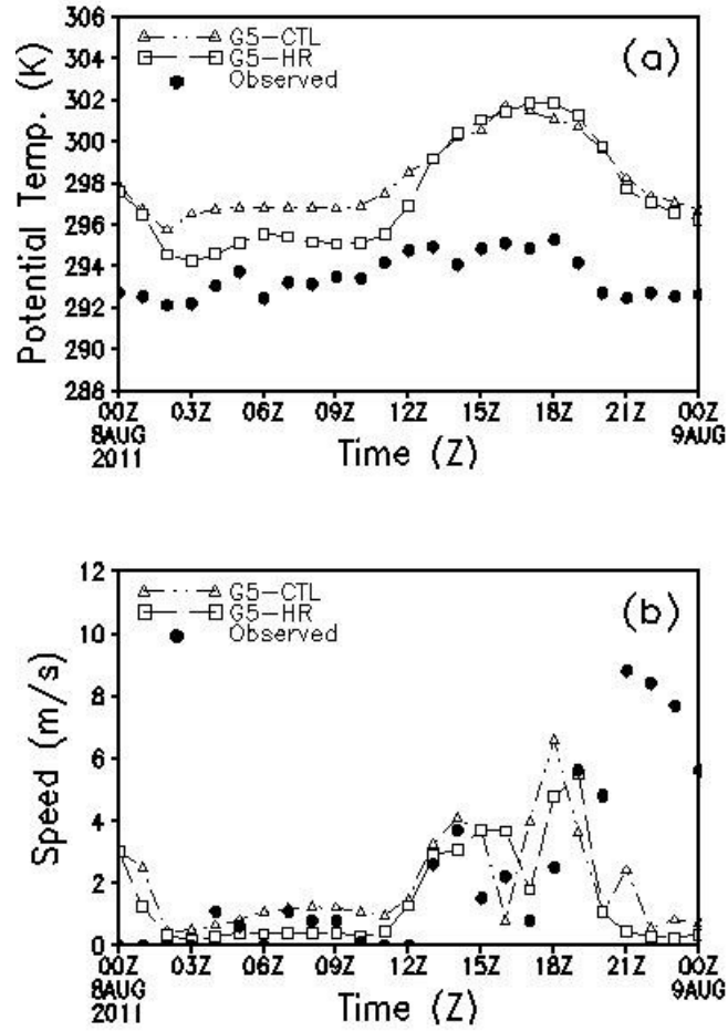
3 Figure 12. Time cross-section data of (a) potential temperature \theta (K), and (b) wind speed (m 4 s^{-1} ) observed (closed circle) and simulated by G5 of CTL (open triangle) and HR (open 5 square) runs for 00:00 UTC 08 August to 00:00 UTC 09 August 2011 at Xerem surface 6 weather-observation station.
