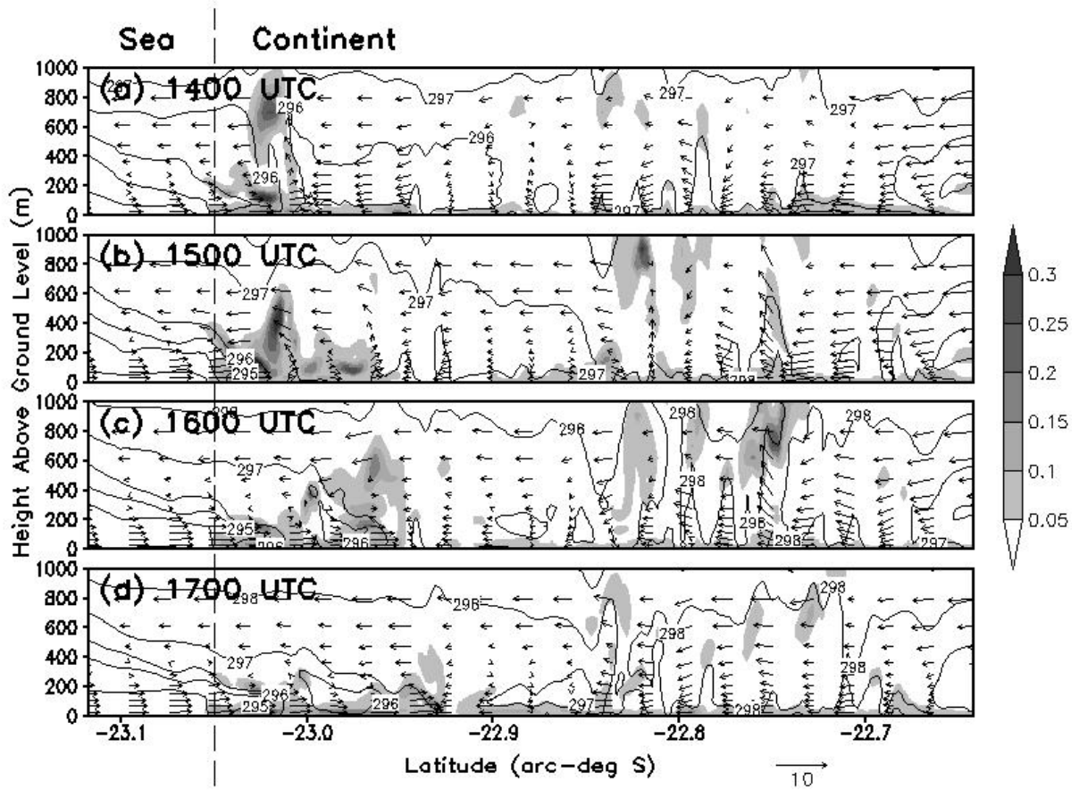
3 Figure 16. Vertical-latitude cross-section of Turbulent Kinetic Energy ( \text{m}^2 \text{s}^{-2} – 4 shaded areas), potential temperature (K – solid line) and meridional-vertical wind vector 5 components ( \text{m s}^{-1} - vectors) up to 1.0 km AGL at -43.60 arc-deg west-longitude (Marambaia 6 longitude location). Values calculated on G5 for the HR run at (a) 14:00 UTC, (b) 15:00 7 UTC, (c) 16:00 UTC and (d) 17:00 UTC 07 September 2007.
