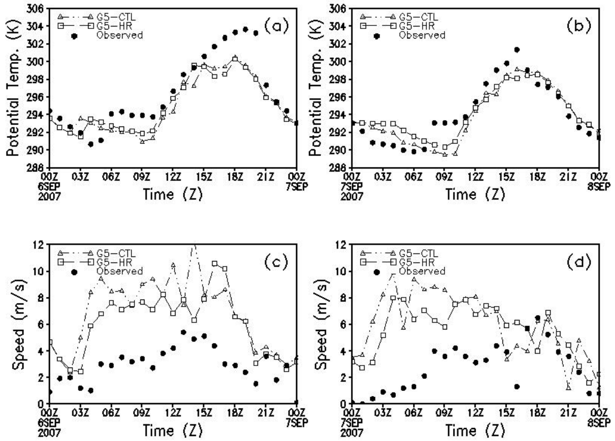
3 Figure 8. Time cross-section data of (a-b) potential temperature \theta (K), and (c-d) wind speed 4 ( \text{m s}^{-1} ) observed (closed circle) and simulated by G5 of CTL (open triangle) and HR (open 5 square) runs for 00:00 UTC 06 September to 00:00 UTC 08 September 2007 at Ecologia 6 Agricola surface weather-observation station.
