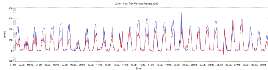
Fig. 8. Surface latent heat flux in Merken in August 2009 at 3 cm depth. Colors as in Fig. 7.
