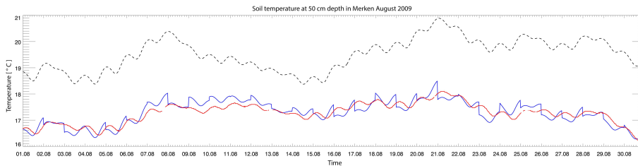
Fig. 5. Soil temperature in Merken in August 2009 at 50 cm depth. Colors as in Fig. 4.
