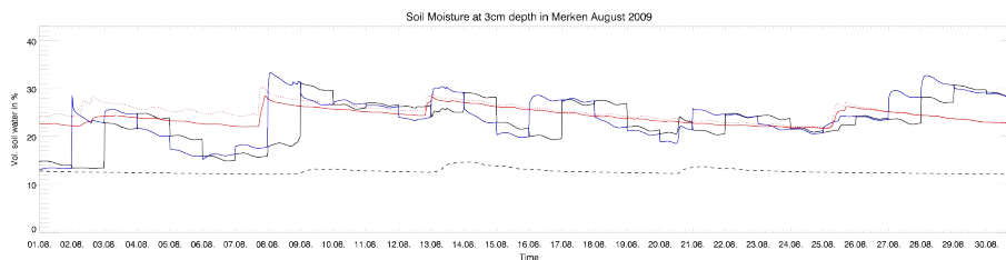
Fig. 6. Soil moisture in Merken in August 2009 at 3 cm depth. The red dotted line displays values of a further instrument (see text). Otherwise, colors as in Fig. 4.
