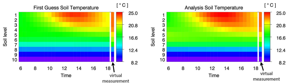
Fig. 2. Time development of soil temperature profile: CLM forecast without assimilation: background run (left panel) and analysis (right panel). In each panel, the separated columns next to the 18:00 temperature profile depict the virtual measurements in soil layers 1–7.
