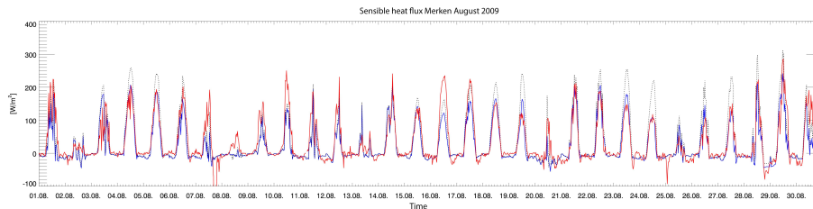
Fig. 7. Surface sensible heat flux in August 2009 at 3 cm depth. The black-dotted curve shows the CLM forecast without assimilation (control run), and the blue curve shows the analysis. Measurements are plotted in red.
