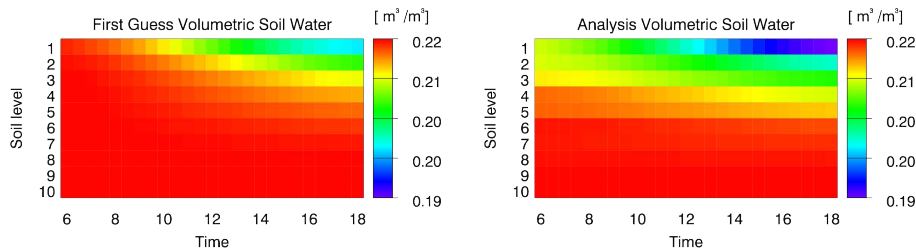
Fig. 3. Time development of soil moisture profile: CLM forecast without assimilation: background run (left panel) and analysis (right panel).
