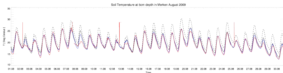
Fig. 4. Soil temperature in Merken in August 2009 at 5 cm depth. The black-dashed curve shows the control run, the black solid curve shows the CLM forecast based on the analysis of the previous day, while the blue curve depicts the analysis. Measurement values are shown as red line.
