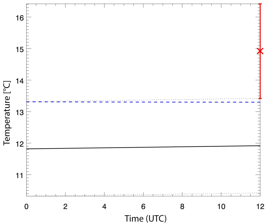
Fig. 1. Assimilation of a virtual soil temperature observation in soil level 9 (172 cm depth) at the end of an assimilation interval of 12 h. The black curve shows the background result and the blue dashed line shows the analysis. The observation is displayed in red.
