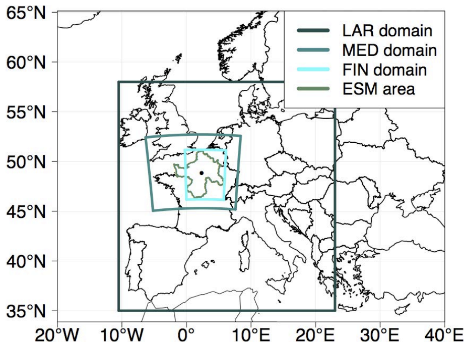
Fig. 1. Nested domains used for the simulations, and ESM area of the bottom-up anthropogenic emission inventory.
