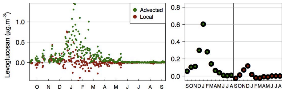
Fig. 11. Daily (left panel) and monthly (right panel) advected (green) and local (red) levoglucosan contributions.
