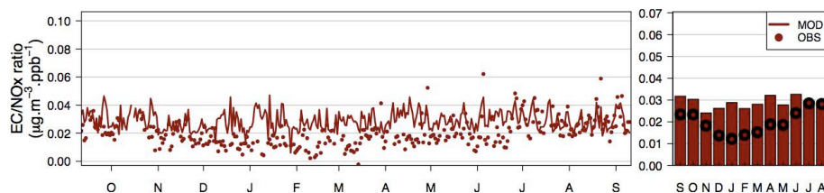
Fig. 10. Local EC/NO x ratio time series (left) and monthly averages (right) for model (line and bar) and observations (points).
