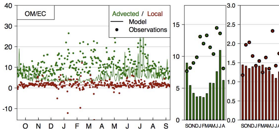
Fig. 12. Local OM/EC ratio (unitless) time series (left) and monthly averages (right) for model (line and bars) and observations (points).
