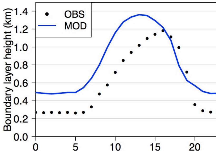
Fig. 5. Boundary layer height diurnal profile at SIRTa station, measured (in black) and simulated (in blue) during the PARTICULES campaign.
