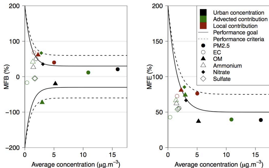
Fig. 13. Mean fractional bias (left panel) and mean fractional error (right panel) depending on the average concentration defined as the average of the mean observed and the mean simulated concentration. Urban background concentrations, advected and local contributions of PM 2.5 and all its compounds are reported, as well as performance criteria (dotted line) and goal (continuous line). Secondary inorganics local contributions are not reported on the graph (see text).
