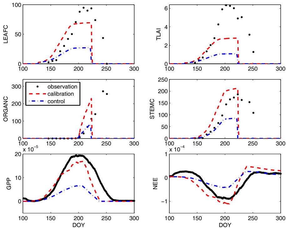
Fig. 2. Calibration results: the observations, the control output, and the calibrated output of 2004.
