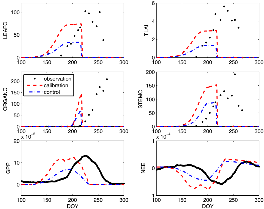
Fig. 3. Validation results: the observations, the control output, and the calibrated output of 2002.
