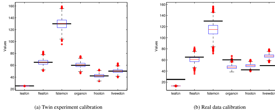
Fig. 1. Calibrated C/N parameters for 2004 for (a) the twin experiment using artificial observations and (b) the real data calibration. The solid black line indicates the default values, and the thin red line indicates the median value for the parameter posterior distribution. The median value was used as the final calibrated parameter value.
