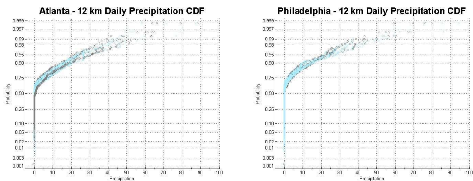
Figure s2. Cumulative distribution of 12 km historic (dark) and future (light) daily precipitation in Atlanta (Left) and Philadelphia (Right).
