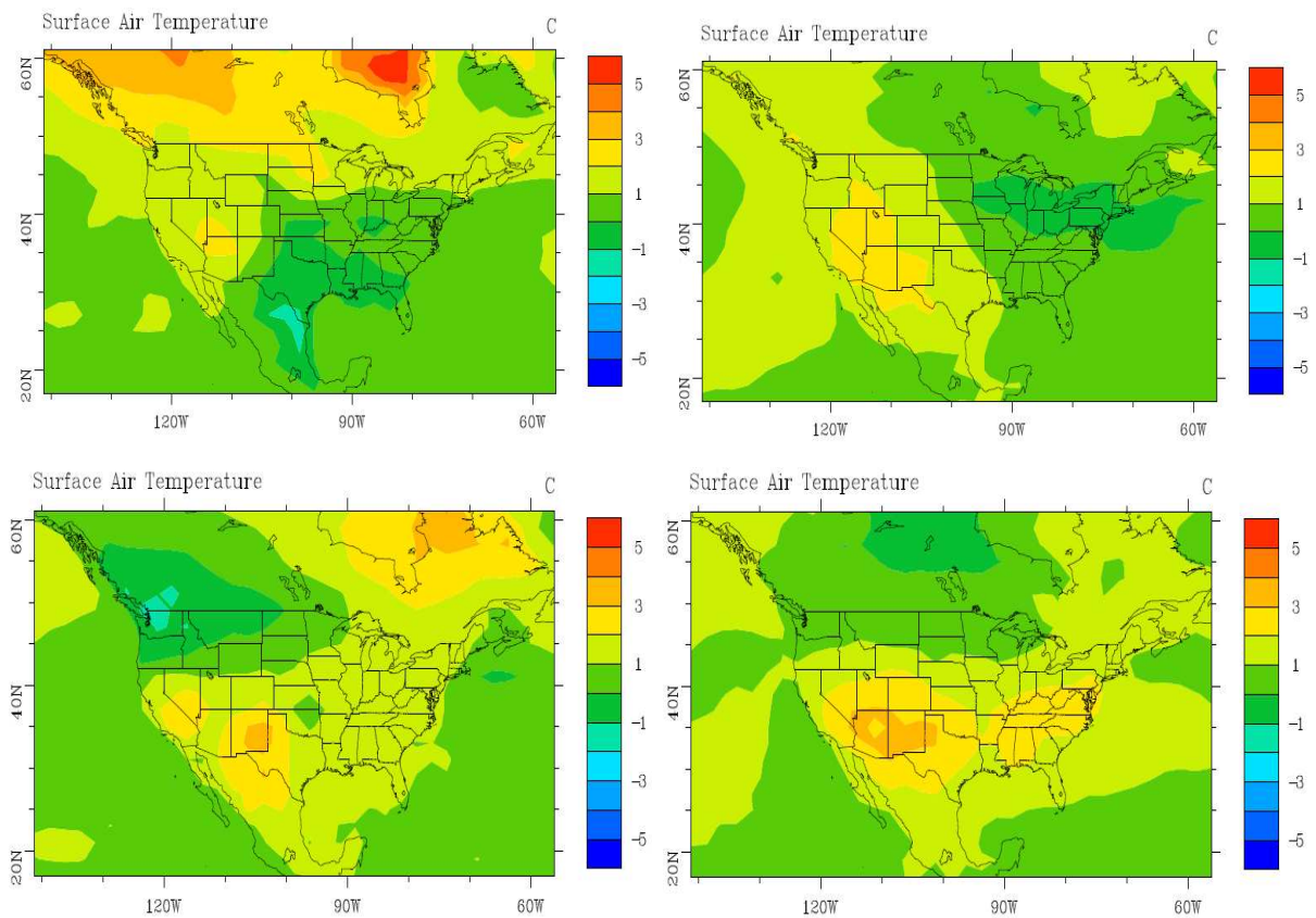
Figure s1. Seasonal GISS GCM surface air temperature (SAT) difference: winter (top left), spring (top right), summer (bottom left), fall (bottom right).
