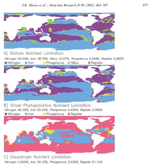
Fig. 8. Nutrient-limitation patterns for the diatoms (A), the small phytoplankton (B), and the diazotrophs (C) during summer months. Areas where all nutrient cell quotas are >97% of the maximum cell quota values are arbitrarily defined as nutrient-replete. Also shown is the percentage of total ocean area where each nutrient is limiting growth.
