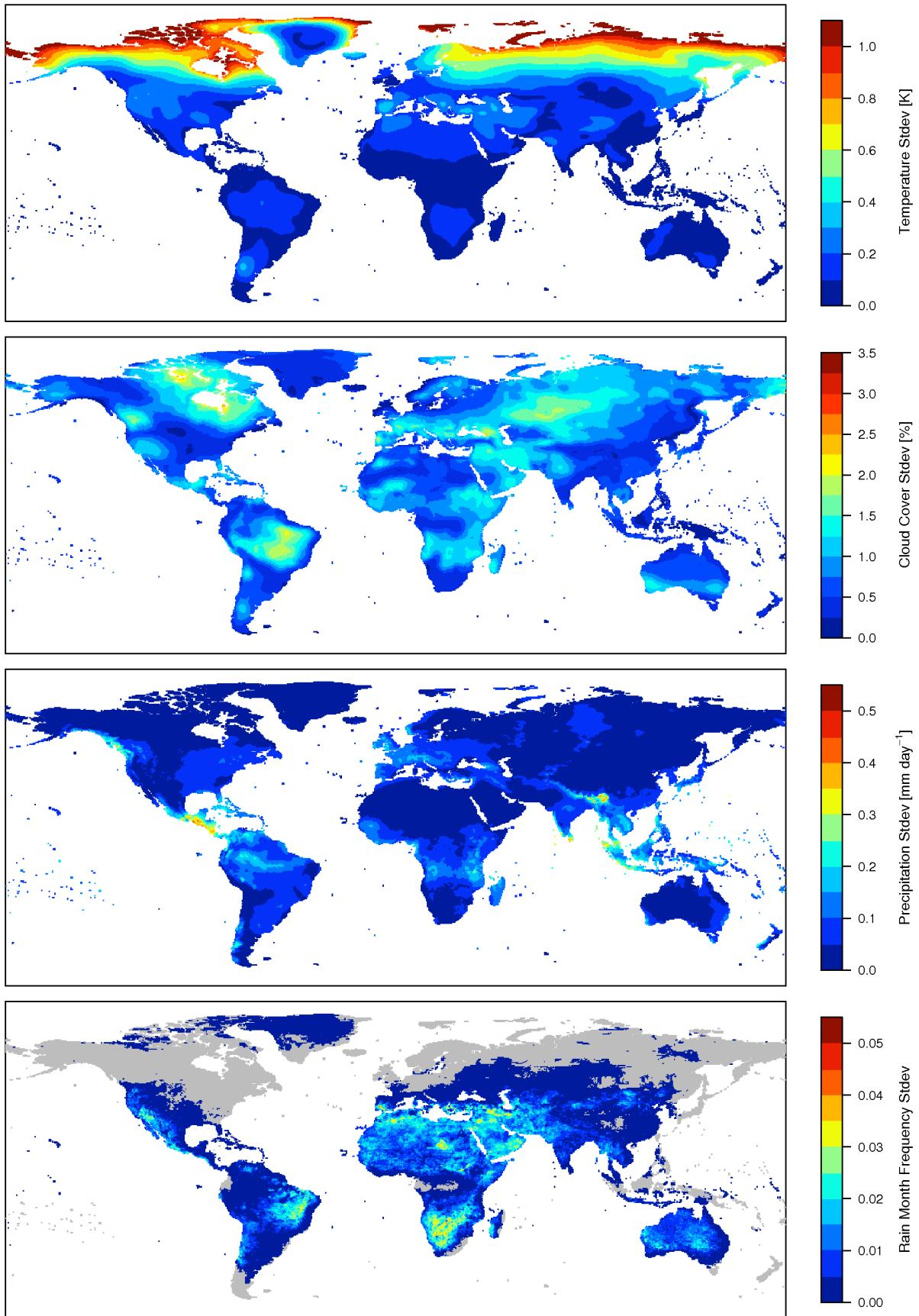
Supplementary Figure 2. Seasonality of change for a 1-degree increase in global mean temperature expressed by the standard deviation of monthly mean anomalies (averaged over all AOGCMs).
