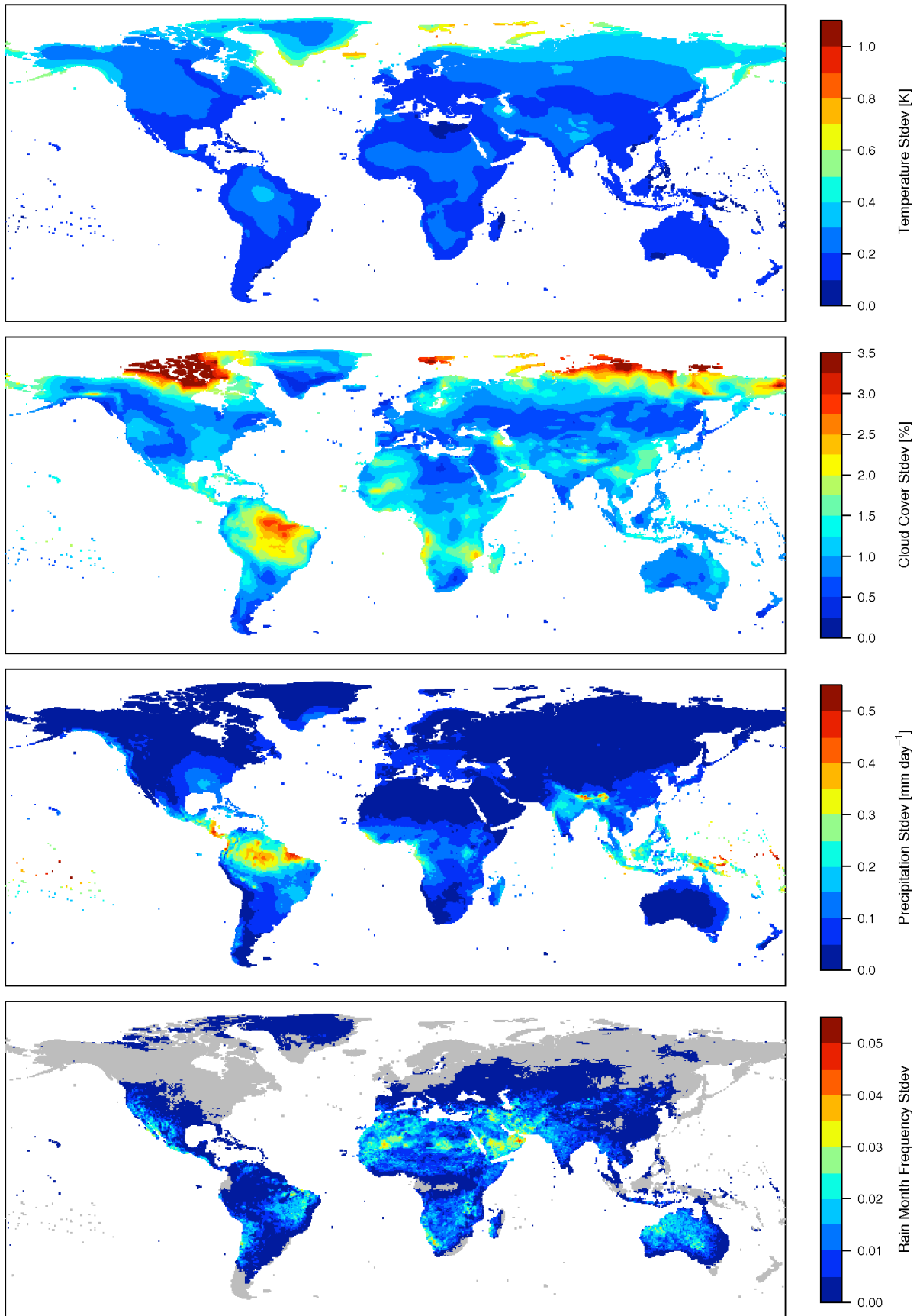
Supplementary Figure 1. Inter-model standard deviation of mean annual change for a 1-degree increase in global mean temperature over all AOGCMs.
