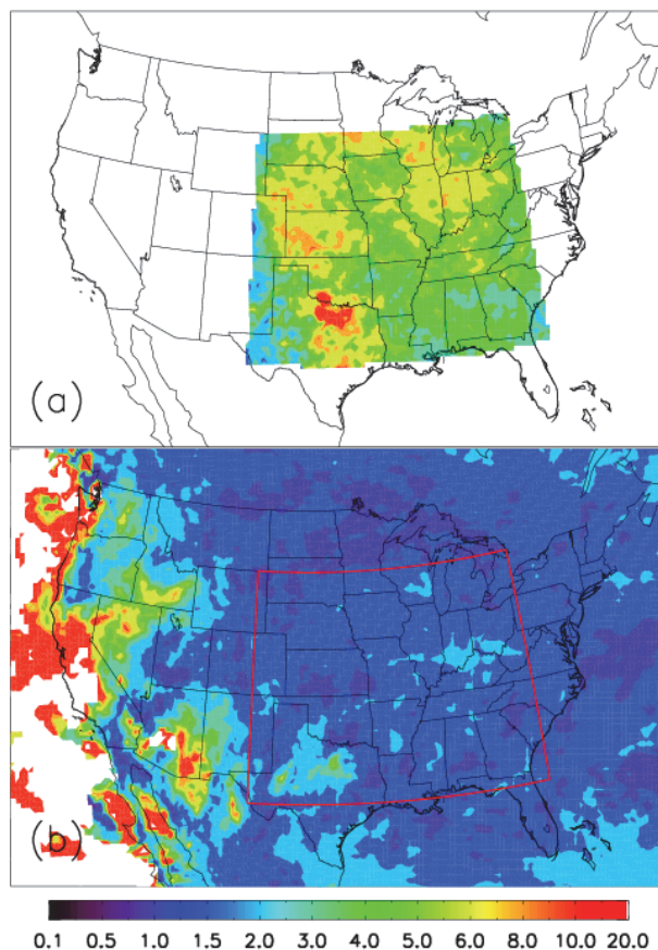
Fig. 8. IC : CG bulk ratios for JJA 2011 as (a) observed by ENTNL and (b) predicted by WRF at 36 km grid spacing using PR93. The ENTNL detection efficiency used here are 0.65 for IC and 0.95 for CG.
