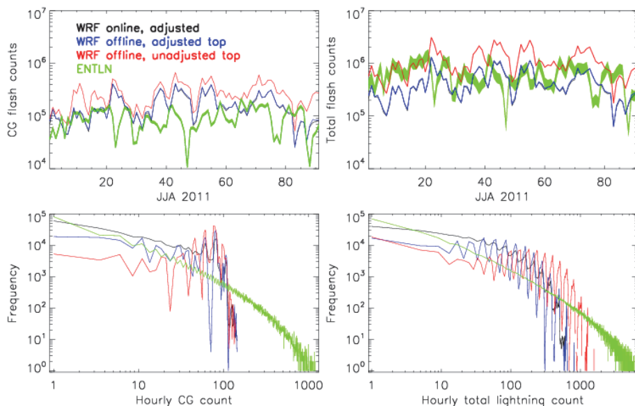
Fig. 9. Comparison of WRF predicted lightning flash counts generated online and offline with and without -2\text{ km} cloud-top height adjustments against ENTLN CG and total flash counts. Thicknesses of the ENTLN bands in the time series are computed using the minimum and maximum theoretical IC and CG detection efficiencies within the analysis domain. Noisiness of offline calculated distributions are associated with using hourly outputs only rather than accumulating flashes at every model time step.
