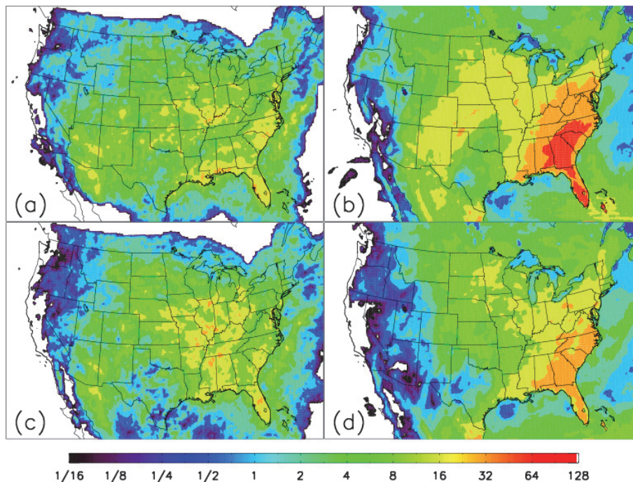
Fig. 4. Total CG flashes in number per \text{km}^2 per full-year during JJA 2006 (first row) and 2011 (second row). First column ( a and c ) shows the NLDN observed density gridded to WRF 36 model grid, and second column ( b and d ) shows the modeled flash density output by WRF at 36 km.
