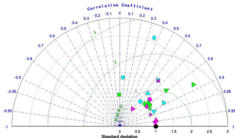
Fig. 2. Taylor diagram of non-area weighted statistical summary between the simulated and observed annually-averaged (climatology) of ( \nabla ) ocean temperature, ( \triangleright ) salinity, ( * ) phosphate, ( \Delta ) dissolved oxygen, ( \circ ) silicate, ( \diamond ) dissolved inorganic carbon, and ( \square ) alkalinity. Shown here are comparison at surface (magenta), 1000 m (blue), and 3000 m (green) depths. Observations are based on the World Ocean Atlas (WOA) and GLODAP (see also text). The black circle represents the observations. All standard deviations are normalized to the respected observed standard deviation. For temperature, salinity, phosphate, silicate and oxygen, we compare the HIST simulation from 1980–1999 period, whereas for DIC and ALK, we use the 1996–2005 simulation period.
