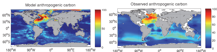
Fig. 13. Maps of anthropogenic carbon inventory for the 1994 period as estimated by the model (left) together with the observational based estimates (right) of Key et al. (2004). Units are in ( \text{molCm}^{-2} ).
