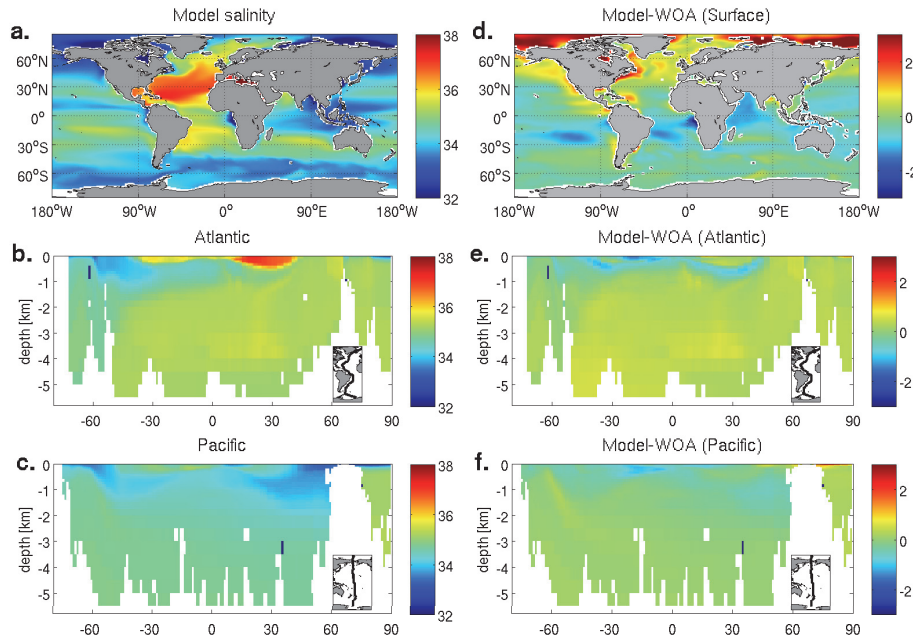
Fig. 4. Distribution of ocean salinity from model simulation (left) and difference in salinity between the model and climatological estimates (right) (WOA, Antonov et al., 2010) for the surface ( a, d ), Atlantic ( b, e ) and Pacific ( c, f ) vertical sections. Units are in (psu).
