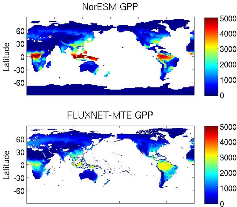
Fig. 15. Maps of mean annual terrestrial gross primary production as simulated by the NorESM model (top) and as estimated from the FLUXNET-MTE observation (bottom). Values are computed from historical 1982–2005 period. Units are in (\text{gC m}^{-2} \text{yr}^{-1}) .
