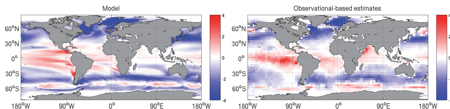
Fig. 11. Maps of annual mean sea-to-air CO 2 fluxes for the 1996–2005 period simulated by the model (left) as compared to the observational based estimates (right) of Takahashi et al. (2009). Units are in (molCm -2 yr -1 ).
