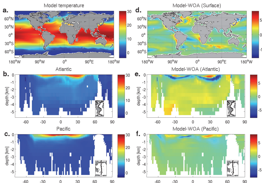
Fig. 3. Distribution of ocean temperature from model simulation (left) and difference in temperature between the model and climatological estimates (right) (WOA, Locarnini et al., 2010) for the surface (a, d), Atlantic (b, e) and Pacific (c, f) vertical sections. Units are in (°C).
