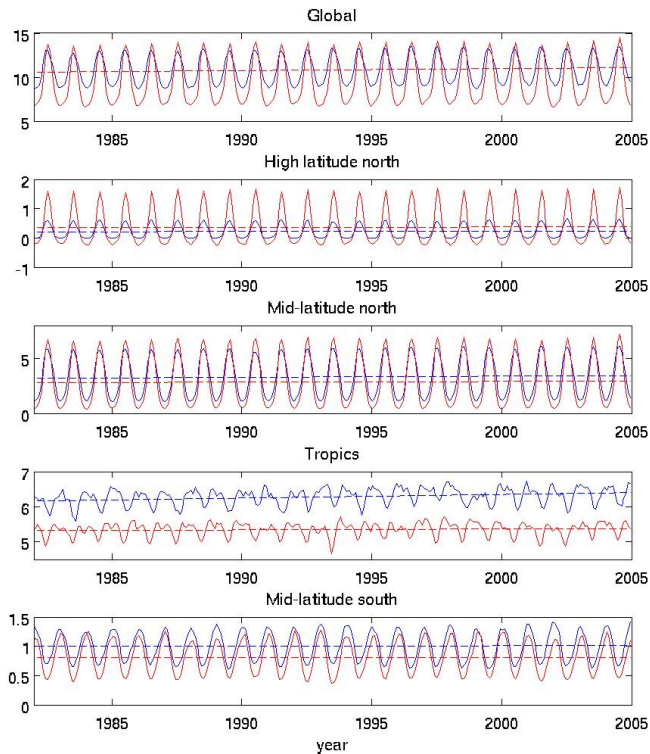
Fig. 17. Time-series of monthly gross primary production (GPP) values simulated by NorESM (blue-lines) as compared to the FLUXNET-MTE estimations (red-lines). Shown are global value, high latitudes ( > 60^\circ \text{N} ), mid-latitude north (between 60^\circ \text{N} and 20^\circ \text{N} ), tropics (between 20^\circ \text{N} and 20^\circ \text{S} ), and mid-latitude south (between 20^\circ \text{S} and 60^\circ \text{S} ). The dashed-lines represent the linear trend of the time-series. Units are in ( \text{PgCmonth}^{-1} ).
