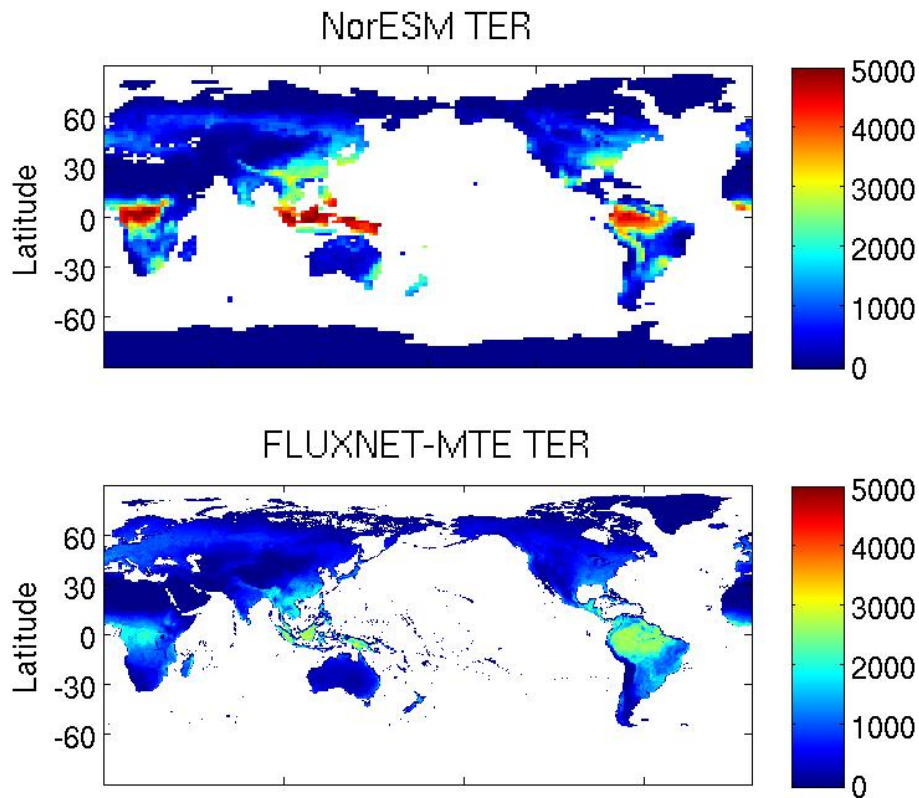
Fig. 16. Same as Fig. 15 for terrestrial ecosystem respiration. Units are in (\text{gCm}^{-2}\text{yr}^{-1}) .
