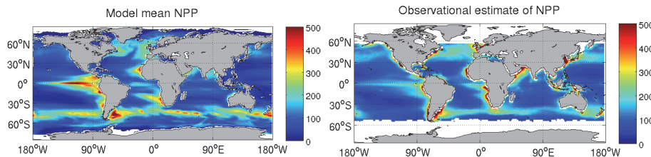
Fig. 9. Model simulated (left) and observed (right) annual mean of surface net primary production. The observation estimate is based on remotely sensed chlorophyll data and the Vertically Generalized Production Model (VGPM) from Behrenfeld and Falkowski (1997). Model value is taken from HIST simulation over 1996–2005 period, whereas the data is from 2003–2007 period. Units are in (\text{gCm}^{-2}\text{yr}^{-1}) .
