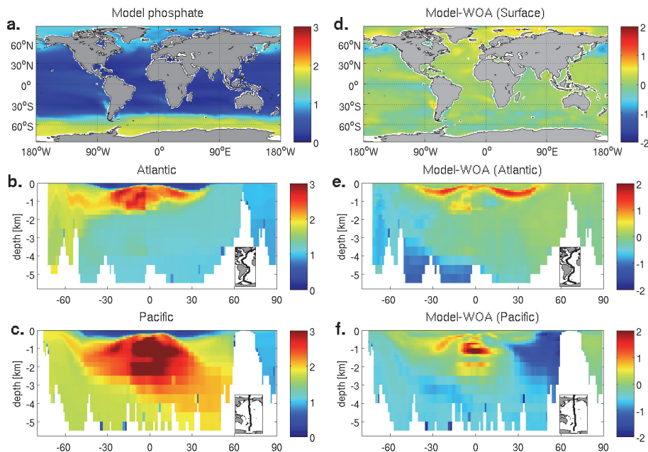
Fig. 6. Distribution of dissolved phosphate concentration from model simulation (left) and difference in phosphate between the model and climatological estimates (right) (WOA, Garcia et al., 2010b) for the surface ( a, d ), Atlantic ( b, e ) and Pacific ( c, f ) vertical sections. Units are in (\mu\text{mol l}^{-1}) .
