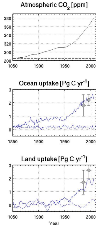
Fig. 12. Time series of atmospheric CO 2 concentration (upper panel), annual oceanic carbon uptake (middle panel), and land (bottom panel) carbon uptake (excluding land use change) simulated over the historical period. Solid lines represent value from HIST, whereas dashed lines represent value from CTRL (shown here only for the first 156 years) simulations. Five-years running mean are applied to the land uptake fields. The observation estimates (grey circles) are from Denman et al. (2007).
