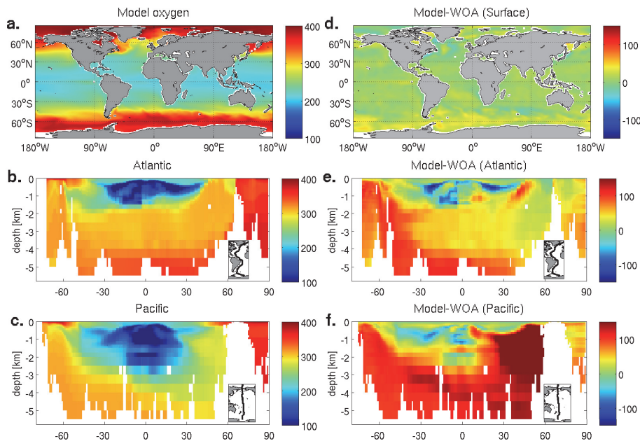
Fig. 7. Distribution of dissolved oxygen concentration from model simulation (left) and difference in oxygen between the model and climatological estimates (right) (WOA, Garcia et al., 2010a) for the surface ( a, d ), Atlantic ( b, e ) and Pacific ( c, f ) vertical sections. Units are in ( \mu\text{mol l}^{-1} ).
