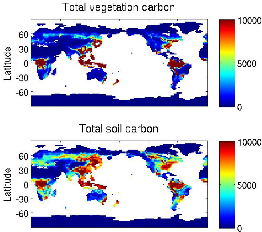
Fig. 14. Maps of mean (top) vegetation and (bottom) soil carbon contents as simulated by the NorESM model. Values are computed over the historical simulation from 1982–2005 period. Units are in (\text{gCm}^{-2}) .
