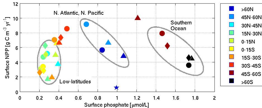
Fig. 10. Latitudinal mean of biological production as a function of mean surface phosphate concentration. The symbols represent different ocean basins: (*) Arctic, (O) Atlantic, ( \Delta ) Pacific, and ( \diamond ) Indian Ocean basin.
