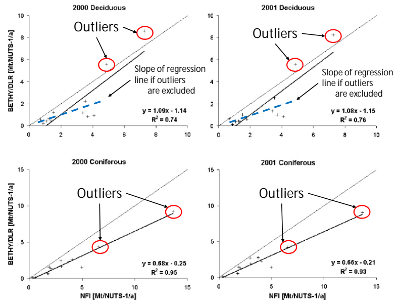
Fig. 1. Outliers in Fig. 4.
