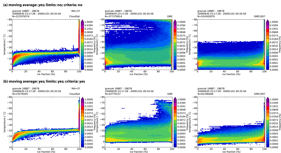
Fig. A: Ice fraction as a function of temperature for 1 July 2009 to 31 October 2009. Left: CloudSat, middle: GME, right: GME1007. Top row (a): no criteria and no limits (according to CloudSat sensitivity range) applied. Bottom row (b): all criteria and IWC and limit applied (temperature not applied). Each data set is normalized with its total number N of included pixel.
