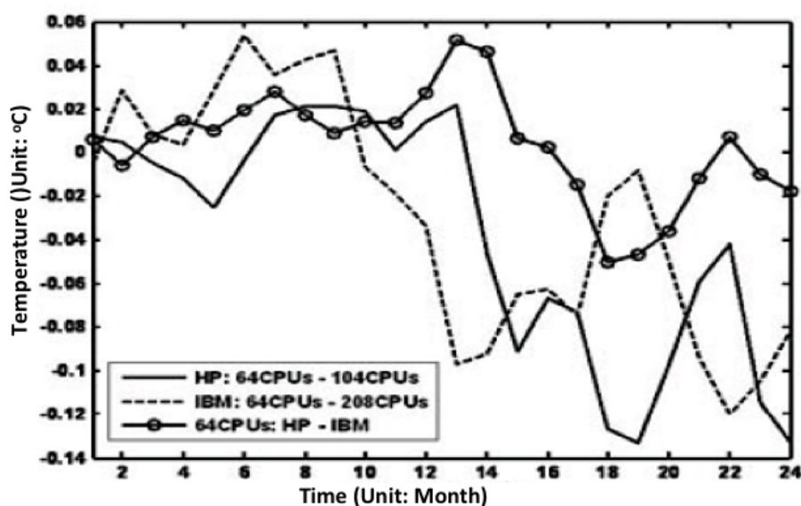
Fig. 1. The Global-SST difference
