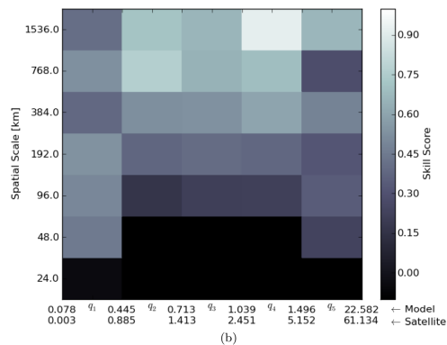
Figure 2: Spatial scales versus quantile ranges plots for May 2004. Sea surface temperature (a) and chlorophyll concentration (b) skill scores.
