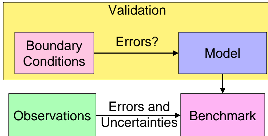
Fig. 2. Sketch of an intercomparison of modelling data to observational data, illustrating the difficulties in attributing discrepancies to model deficiencies rather than input or boundary data uncertainties.
