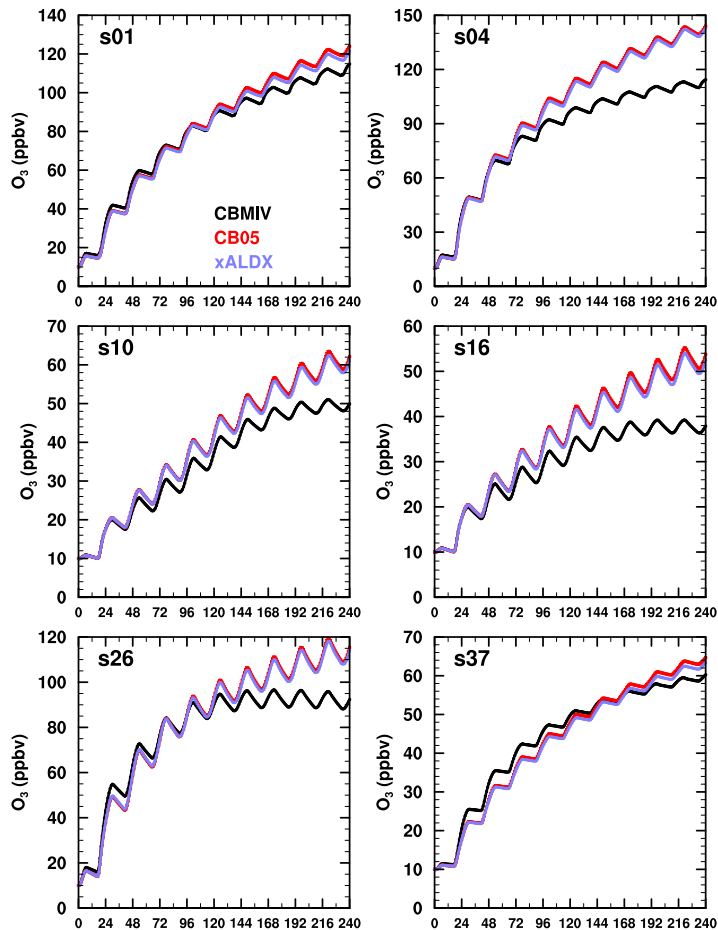
Fig. 3. Example scenario results for sensitivity test xALDX. Ozone mixing ratios (ppbv) for the base CB05 (red), base CBMIV (black) and sensitivity test xALDX (violet) over the 240 h simulation period.
