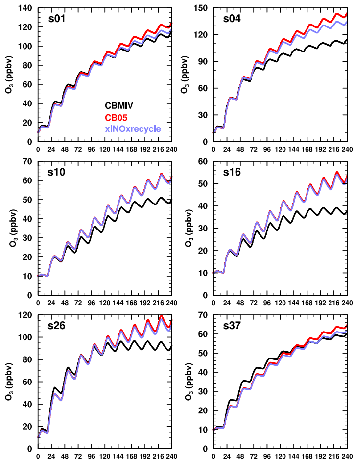
Fig. 8. Example scenario results for sensitivity test xiNOxrecycle. Ozone mixing ratios (ppbv) for the base CB05 (red), base CBMIV (black) and sensitivity test xiNOxrecycle (violet) over the 240 h simulation period.
