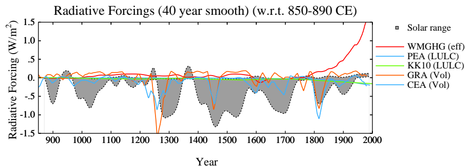
Fig. 4. Estimated radiative forcings for each driver (solar and volcanic forcings are smoothed using a 40 yr triangular filter).
