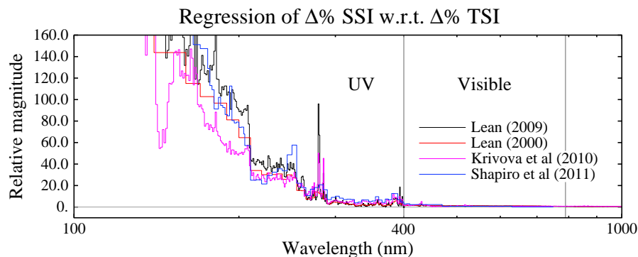
Fig. 3. Ratio of spectral irradiance variability to total solar irradiance variability from UV to Near IR. This shows the regression of the % change in SSI at each wavelength to the % change in TSI for 4 separate estimates (Lean, 2000, 2009; Krivova et al., 2010; Shapiro et al., 2011) (cf. Fig. 7 in Schmidt et al., 2011).
