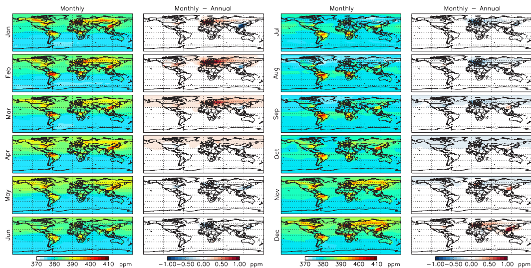
Fig. 1. Comparison of monthly-averaged surface level CO 2 in 2006 from a simulation using the monthly-varying fossil fuel emissions and another run using annual fossil fuel emissions with the same cumulative annual total. The runs began with the same initial conditions for 1 January 2006 and were identical in all other respects.
