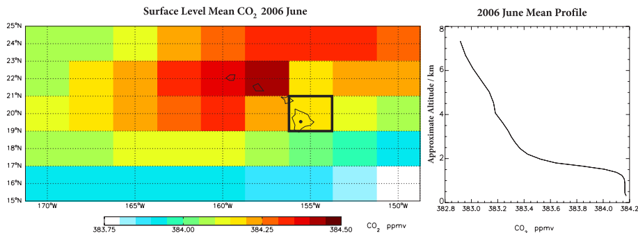
Fig. 11. GEOS-Chem mean surface level CO 2 for 2006 June for the Hawaiian Islands region (left). The CO 2 profile for the gridbox containing Mauna Loa (right) corresponds to the area outlined in black in the left panel. Altitude is only approximate for the profile because it is based on a conversion from model hybrid sigma levels which requires assuming a surface pressure that will vary throughout the gridbox (222 km × 261 km) from sea level to about 4.2 km altitude. The location of the Mauna Loa observatory is shown by the black dot.
