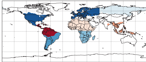
GFEDv2 Biomass Burning Climatology 1997–2006 and 1995 Biofuel Emissions
