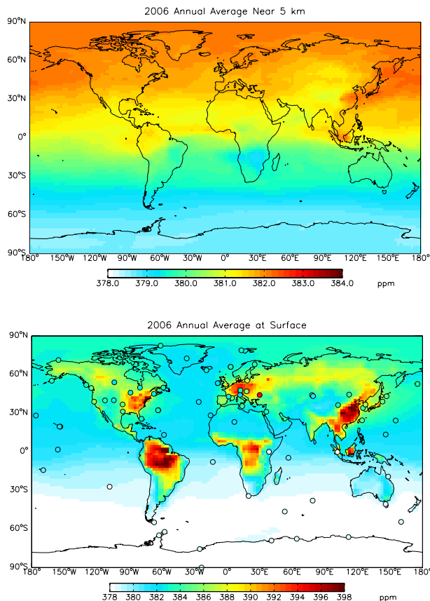
Fig. 10. Annually-averaged 2006 model CO 2 from a run with emissions from shipping, aviation and the chemical source. The upper panel shows CO 2 at the model level near 5 km and the lower panel shows model CO 2 at the surface level compared with 74 GLOBALVIEW-CO 2 stations on the same color scale (colored circles).
