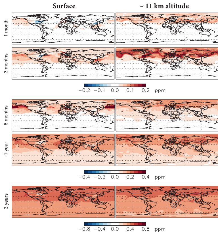
Fig. 4. Combined impact of shipping and aviation emissions on CO 2 at increments up to 3 years at the surface and at the model level near 11 km altitude where aviation emissions peak. The small negative CO 2 changes at the surface (which are most visible in the first month in the US and China) are a result of the correction to the land fossil fuel source to avoid counting emissions from domestic aviation in both inventories.
