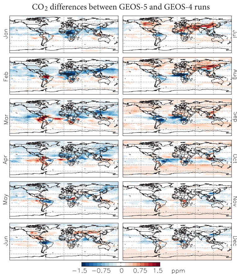
Fig. 16. Monthly-averaged CO 2 difference plots from simulations with different meteorological fields (GEOS-5–GEOS-4) for 2006 at the level near 5 km. The runs began on 1 January 2004 with identical conditions and were exposed to identical fluxes (without the chemical source).
