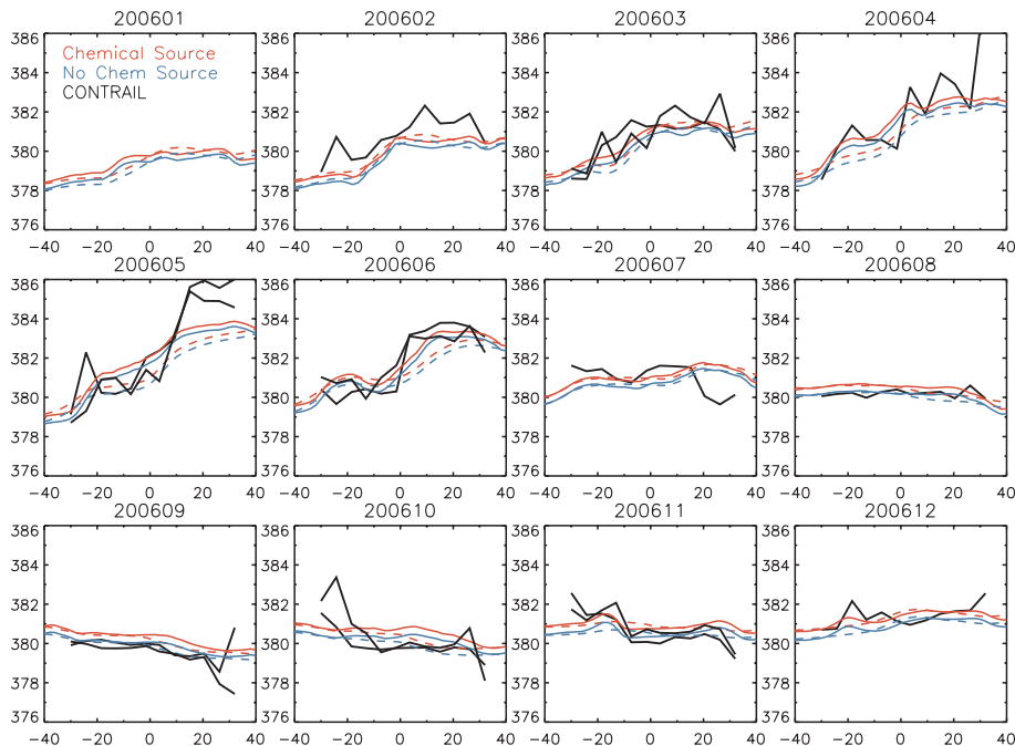
Fig. 15. Model monthly-averaged CO 2 versus latitude at the level near 10 km with the chemical source (red) and without the chemical source (blue) compared with CONTRAIL (black). The solid line shows the model at the mean CONTRAIL longitude (145° E) and the dotted line is a zonal average.
