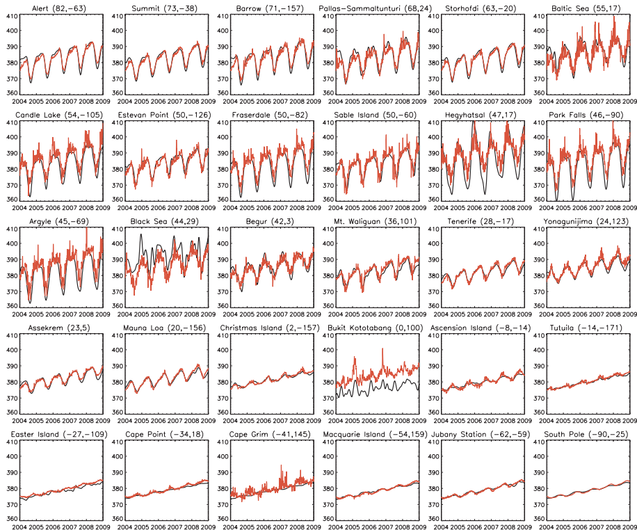
Fig. 12. 7-day averaged GEOS-Chem CO 2 with the chemical source on (red) compared with GLOBALVIEW-CO 2 smoothed ~7.6-day average (black) at 30 stations ranging from 90°S–82°N. The run began with globally-uniform CO 2 at 375.0 ppm on 1 January 2004 causing a visible discrepancy at northern mid and high latitudes at the start of the run, although this is corrected by the model during the first few months.
