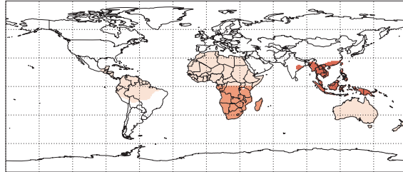
Annual Terrestrial Exchange Climatology (Transcom - Biomass/Biofuel)
