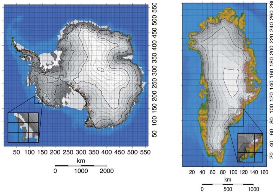
Fig. 7. The numerical grid of AGISM has a horizontal resolution of 10 km for both polar ice sheets (left panel: Antarctic ice sheet; right panel: Greenland ice sheet). Major gridlines are for a distance of 100 km, the insets show the detailed meshes employed in the calculations. The numbers along the axes are gridpoint numbers (561×561 gridpoints for AISM, 165×281 for GISM). The background field is for surface elevation. Ice sheet cover is shaded grey, ice-free areas range from green to white, and blue colours depict the ocean.
