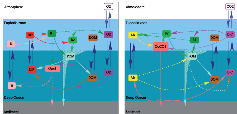
Fig. 5. Schematic representation of the main processes described in the LOCH model (Mouchet, 2010). The left panel focuses on purely biological processes while the right panel shows the processes affecting the ocean carbon cycle. Up and down blue arrows represent transport processes (advection, diffusion, etc.). Transported variables include dissolved inorganic carbon (DIC), alkalinity (Alk), dissolved inorganic phosphorous (DIP), dissolved organic matter (DOM), oxygen (O 2 ), and silica (Si). At the air-sea interface CO 2 and O 2 are exchanged with the atmosphere. B1 stands for opal building phytoplankton biomass, B2 represents the biomass of phytoplankton not relying on silica for growth (please note the inversion of B1 and B2 boxes between panels). POM is distributed at depth according to a power law and decays either as DOM or DIP. Opal dissolves while sinking to the bottom. Calcareous shells (CaCO 3 ) reach the deepest layer where chemical conditions drive their dissolution or preservation. Fluxes toward sediments, where permanent preservation prevails in this version, are also represented. Rivers (not illustrated) carry Si, DOM, DIC and Alk to the ocean.
