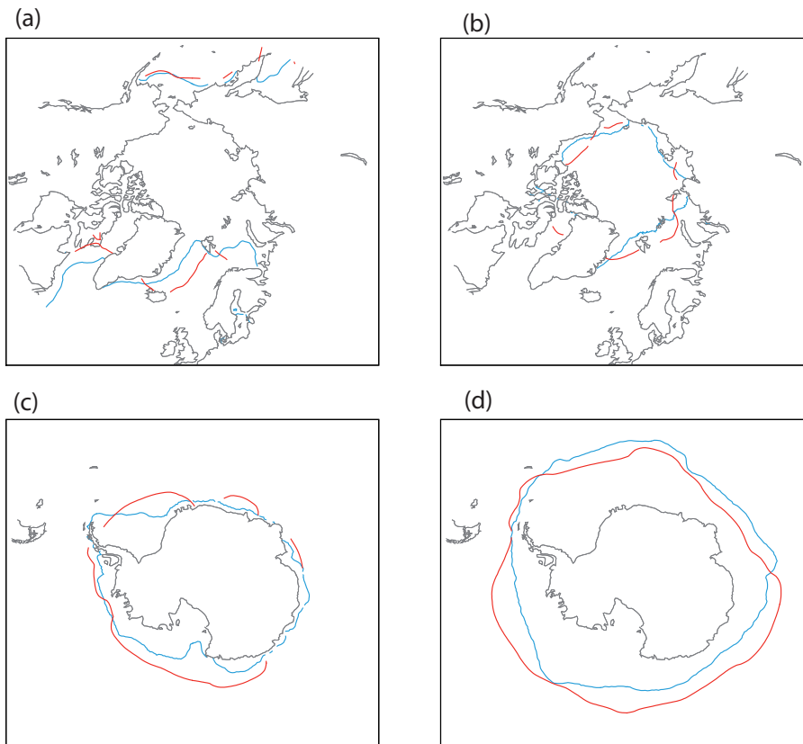
Fig. 12. The location of the ice edge averaged over the period 1980–2000, defined by a monthly ice concentration equal to 15% in (a) March in the Northern Hemisphere, (b) September in the Northern Hemisphere, (c) September in the Southern Hemisphere, (d) March in the Southern Hemisphere. The observations are in blue (Rayner et al., 2003) and LOVECLIM 1.2 results are in red.
