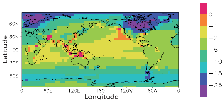
Fig. 20. Difference of annual mean surface temperatures (in °C) between the last glacial maximum and present-day conditions.
