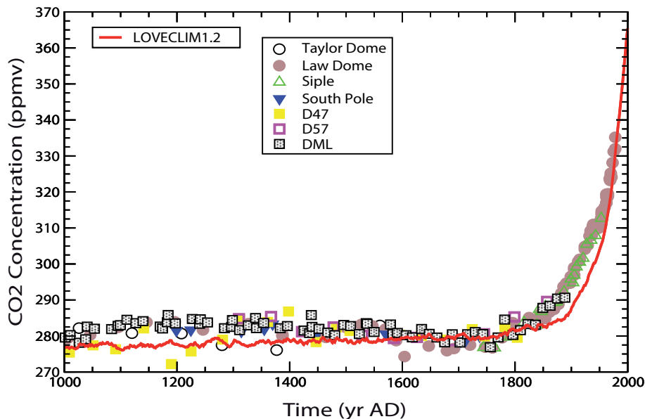
Fig. 16. Atmospheric CO 2 concentration in LOVECLIM 1.2 (red line) compared to measured made in various ice cores: Taylor Dome (Indermühle et al., 1999), Law Dome (Etheridge et al., 1998), Siple (Neftel et al., 1994), South Pole (Siegenthaler et al., 2005), D47 (Barnola et al., 1995), D57 (Barnola et al., 1995), Draening Maud Land (DML, Siegenthaler et al., 2005).
