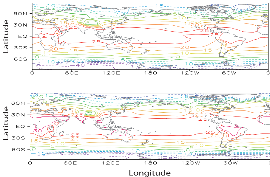
Fig. 9. Surface temperature (°C) averaged over the period 1980–2000 in (a) HADCRUT3 dataset (Brohan et al., 2006) and in (b) LOVECLIM 1.2.
