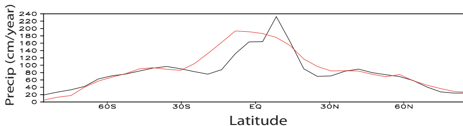
Fig. 10. Zonal mean precipitation (cm/year) averaged over the period 1980–2000 in Xie and Arkin (1996 and updates) dataset (black) and in LOVECLIM 1.2 (red).
