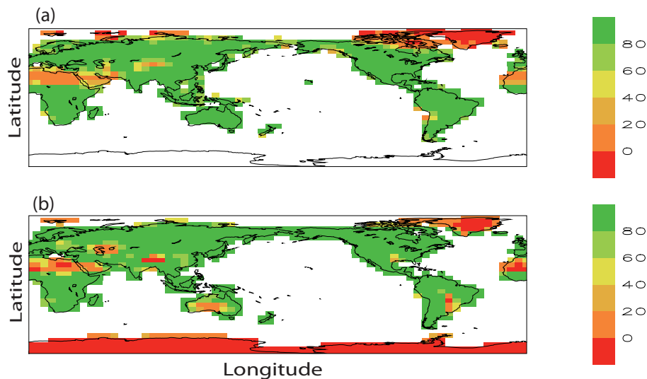
Fig. 14. Total vegetation cover in (a) GSWP2 dataset (International GEWEX Project Office, 2002) and in (b) LOVECLIM 1.2.
