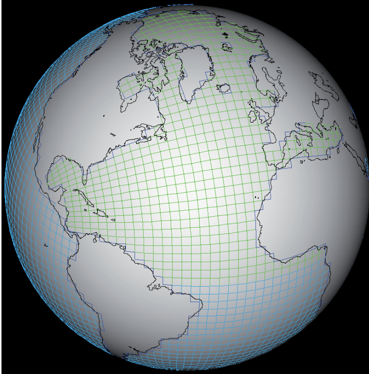
Fig. 4. The horizontal grid of the model at a resolution of 3^\circ by 3^\circ . The view is centred on the Atlantic. The two spherical subgrids in two different colors are connected in the Atlantic at the “geographical equator”.
