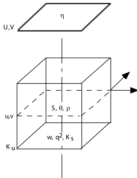
Fig. 3. Location of the various variables on the grid of CLIO. U , V are the two components of the barotropic velocity, \eta the surface elevation, u , v , w , the three components of the velocity, S the salinity, \theta the potential temperature, q^2 (two times) the turbulent kinetic energy, K_s and K_u the vertical diffusion and vertical viscosity.
