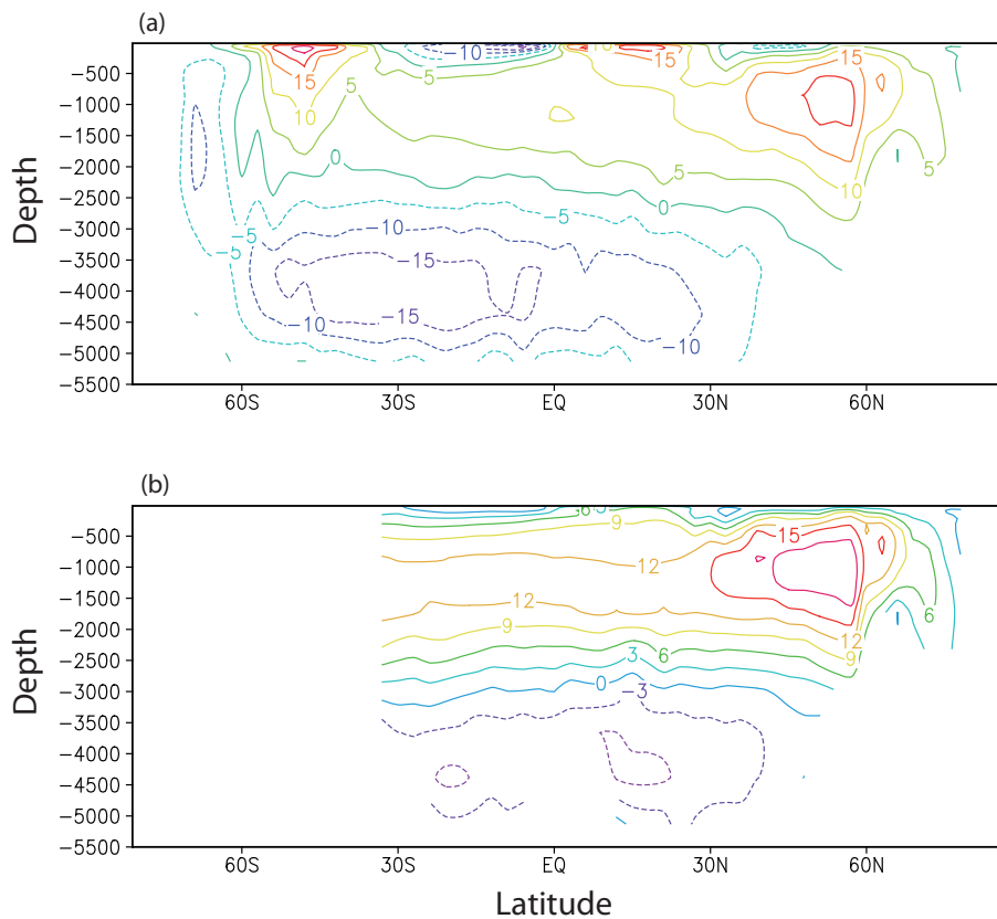
Fig. 13. Meridional overturning streamfunction (in Sv) for (a) the whole World Ocean and (b) the Atlantic.
