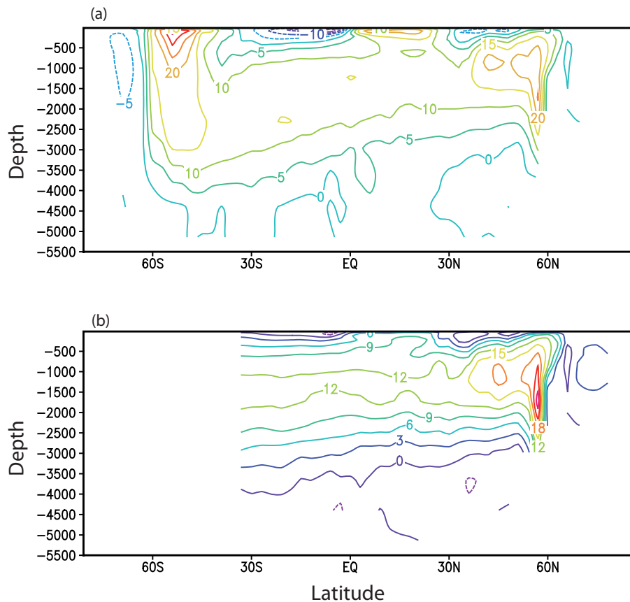
Fig. 21. Meridional overturning streamfunction (in Sv) for (a) the whole World Ocean and (b) the Atlantic simulated for the last glacial maximum.
