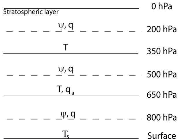
Fig. 2. Vertical discretisation of the atmospheric model ECBilt.
