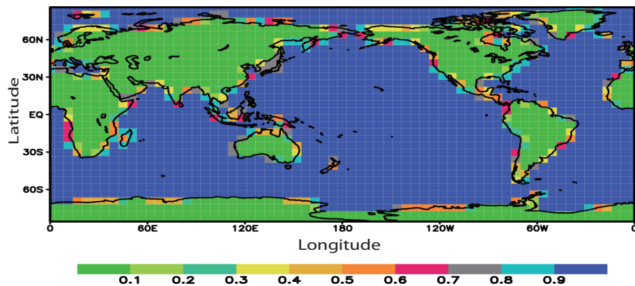
Fig. 8. Fraction of ocean surface in each of the grid points of ECBilt.
