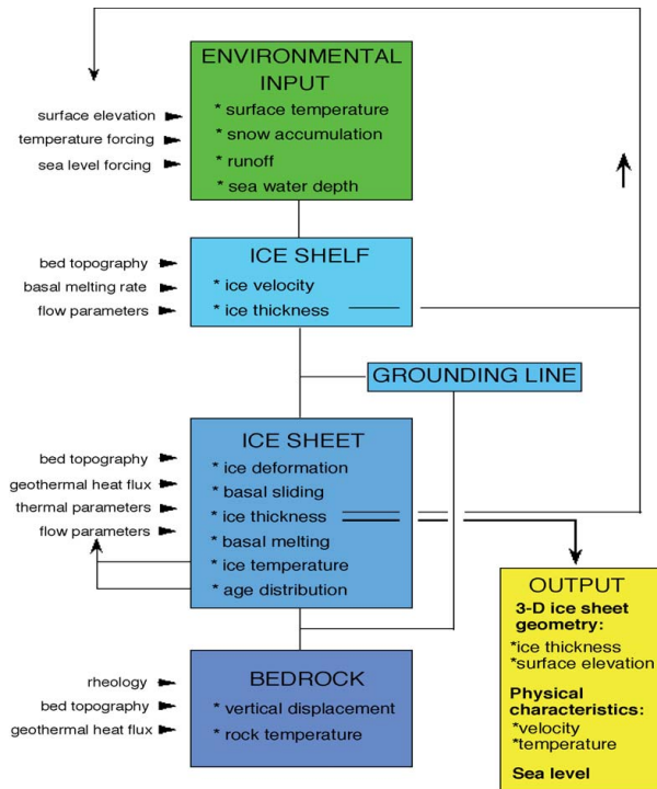
Fig. 6. Structure of the three-dimensional ice-sheet model AGISM. The inputs are given at the left-hand side. Prescribed environmental variables drive the model, which has ice shelves, grounded ice, and bed adjustment as major components. For the Antarctic component, the position of the grounding line follows from a flotation criterion and a specific treatment of the force balance. Ice thickness feeds back on surface elevation, an important parameter for the calculation of the mass balance. The main model outputs the time-dependent ice-sheet geometry and the coupled temperature and velocity fields.
