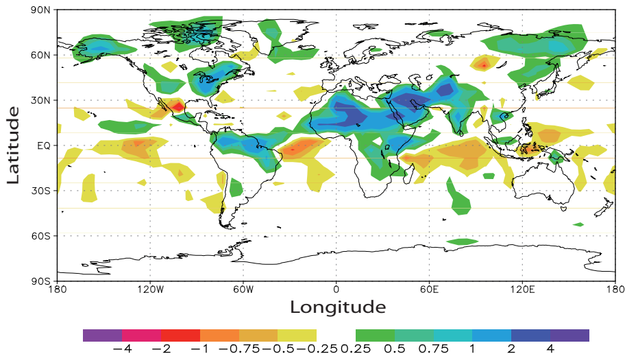
Fig. 19. Difference of summer (JJAS) precipitation (in mm per day) between the mid-Holocene and present-day conditions.
