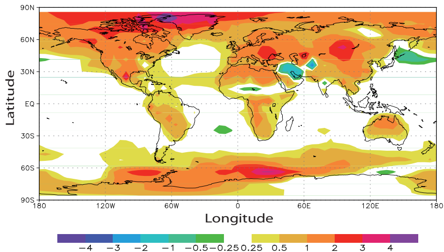
Fig. 18. Difference of summer (JJAS) temperatures (in °C) between the mid-Holocene and present-day conditions.
