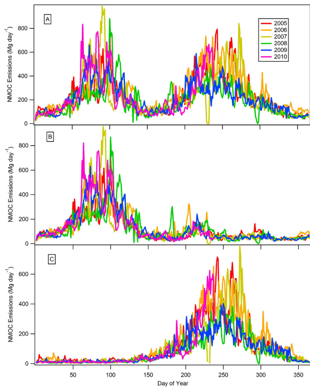
Fig. 2. Daily emissions of NMOC from fires for 2005 through August 27, 2010 for (A) the globe, (B) the Northern Hemisphere, and (C) the Southern Hemisphere.
