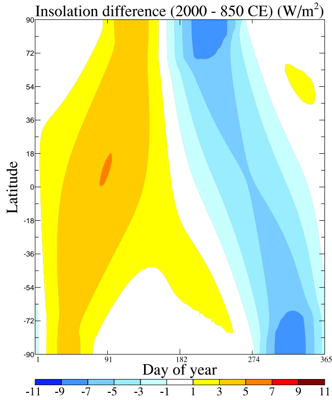
Fig. 1. Insolation difference (2000–850 CE) ( W/m^2 ) as a function of latitude and Julian day.
