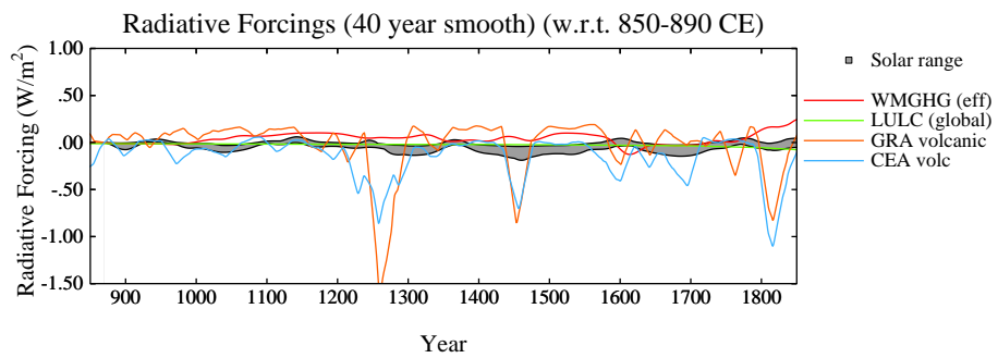
Fig. 9. Radiative forcing from well-mixed greenhouse gases (using the IPCC formulas and efficacy from Hansen et al., 2005), LULC-related albedo change (Pongratz et al., 2009), a smoothed envelope of solar forcing, and the two smoothed volcanic reconstructions. Smoothing is with a 40-year triangular filter.
