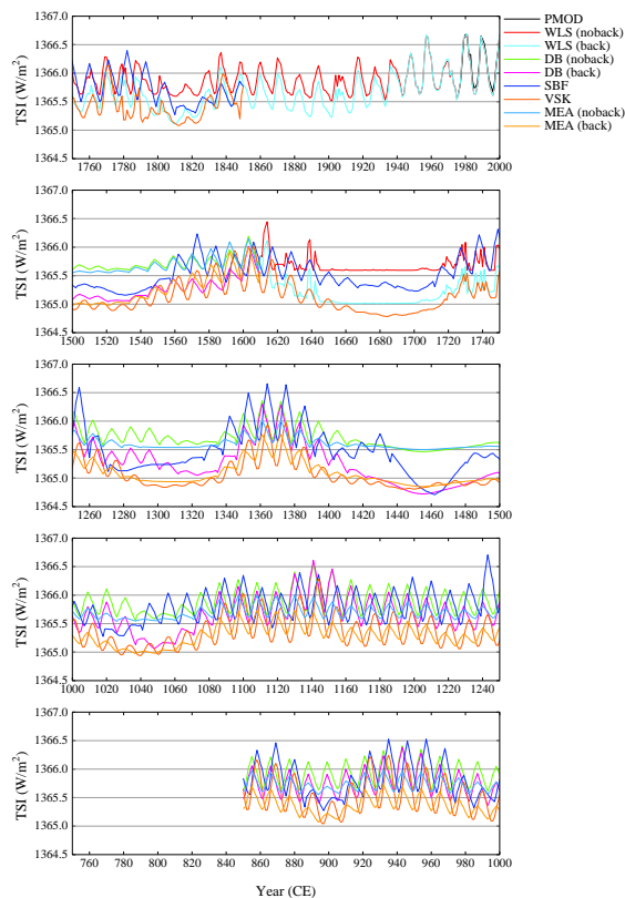
Fig. 8. Multiple TSI reconstructions from 850 CE onwards.
