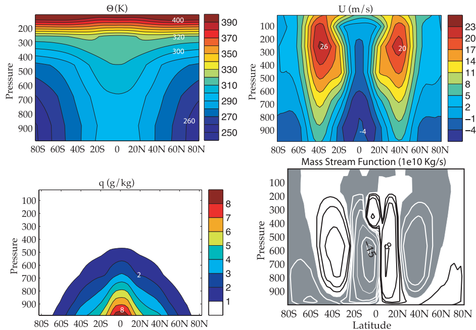
Fig. 11. Zonal mean atmospheric potential temperature \Theta , zonal wind U , humidity q and mass streamfunction \psi_a in the sector atmosphere. The jet is stronger in the Southern Hemisphere and projects onto stronger surface westerlies; the southern Hadley cell is also stronger and penetrates across the equator. From the depth of the Ferrel cells we can see that the planetary boundary layer is very deep due to relative too warm land over half of the domain. Note that there is no seasonal cycle in the model.
