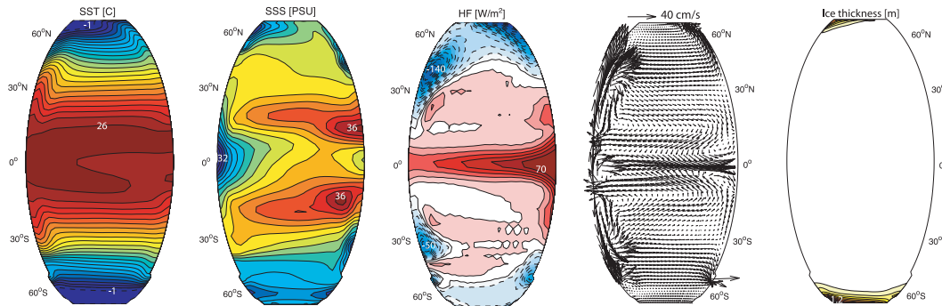
Fig. 6. Sea surface temperature (SST), salinity (SSS), heat flux (HF), 100-m-averaged mean oceanic currents and sea-ice thickness in the Atlantic experiment. The contour interval is 1^{\circ}\text{C} for temperature, 0.25 psu for salinity and 10\text{ W m}^{-2} for the surface heat flux and 0.1 m for sea-ice; a reference velocity arrow is given at the top of the fourth panel for velocity reference. Many aspects of the mean state oceanic conditions can be interpreted from these panels: an equatorial cold tongue is present, sea-ice concentration is asymmetric between the poles, surface salinity has two major salty limbs in the subtropics and region of freshwater river discharge are visible. Finally the ocean gains heat in the equatorial region (positive flux is into the ocean) and loses heat to the atmosphere at the poles and in the western boundary current areas.
