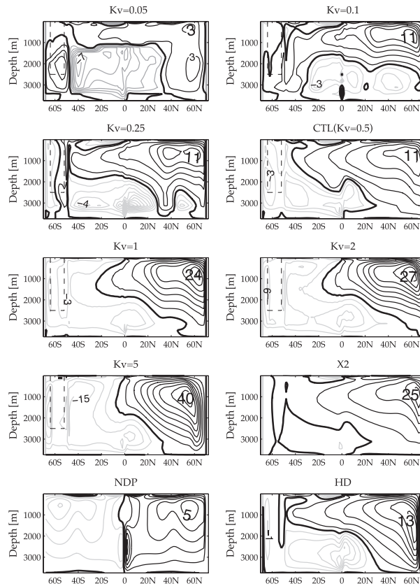
Fig. 8. The time-mean residual meridional overturning circulation in Sverdrups ( Sv \equiv 10^6 \text{ m}^3/\text{s} ) in the different coupled experiments for different values of vertical diffusivity ( \kappa_v , in \text{m}^2\text{s}^{-1} ), basin width (X2, two times wider), no Drake Passage (NDP, closed basin) and Laplacian horizontal diffusivity (HD, same parameter value as in GM).
