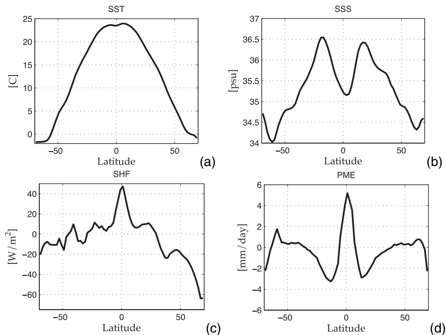
Fig. 2. Surface fluxes in the Atlantic coupled model climatology after spin-up. (a) sea surface temperature (SST) in °C, (b) sea surface salinity (SSS) in PSU, (c) surface heat flux (SHF) into the ocean in \text{W m}^{-2} and (d) precipitation minus evaporation (PME) in mm/day.
