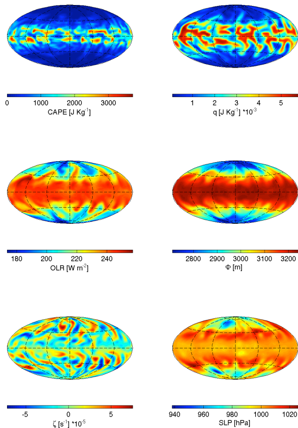
Fig. 16. Daily snapshot of some atmospheric fields for the Aquaworld experiment. From top left: convectively available potential energy (CAPE), specific humidity ( q ) at 500 mb, outgoing longwave radiation (OLR), geopotential height ( \Phi ) at 500 mb, relative vorticity ( \zeta ) at 500 mb and sea level pressure (SLP).
