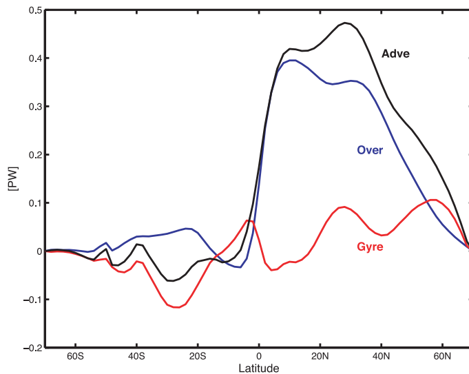
Fig. 10. Meridional oceanic heat transport for the Control (CTL) case ( \kappa_v=0.5\times 10^{-4} ). Advection (black), Overturning (blue) and Gyre (red) component.
