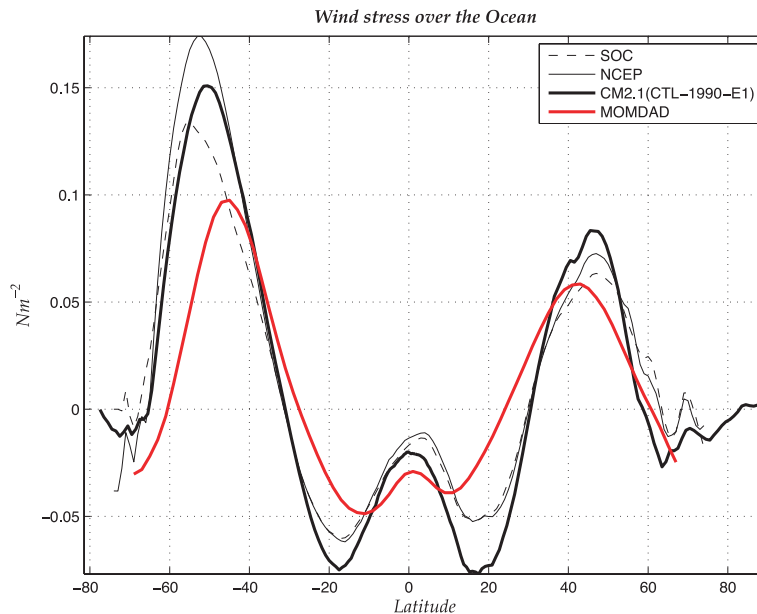
Fig. 3. The wind stress over the ocean for the ICCM model (red line, Atlantic case) and the GFDL CM2.1 (heavy black line). The other two curves are observational data sets. The major deficiencies are a too small difference between the Northern and Southern Hemisphere midlatitude jets, and the equatorward position of the southern midlatitude jet.
