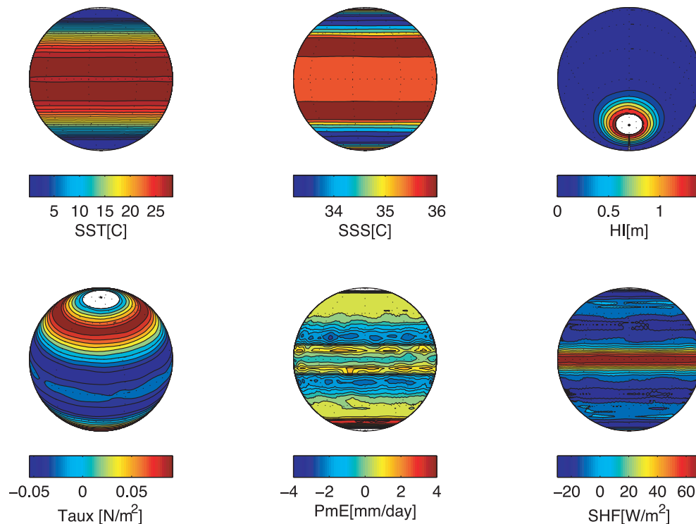
Fig. 14. Some oceanic fields during spin-up of the Aquaworld experiment. From top left: sea surface temperature (SST), sea surface salinity (SSS), sea-ice thickness (HI) in meters, zonal wind stress (Taux) in \text{N m}^{-2} , precipitation minus evaporation (PmE) in \text{mm day}^{-1} and the total surface heat flux (SHF) in \text{W m}^{-2} . The polar islands can be seen in some of the plots.
