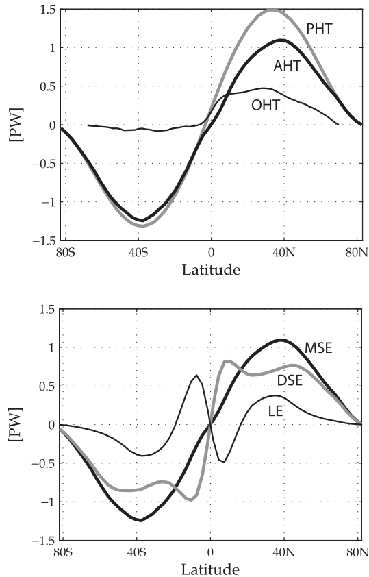
Fig. 12. Top panel: Planetary (PHT), atmospheric (AHT) and oceanic (OHT) heat transport for the sector Atlantic model. Lower panel: AHT or moist static energy ( MSE=C_pT+gz+L ), dry static energy ( DSE=C_pT+gz ) and latent energy ( LE=L ) in the CTL simulation.
