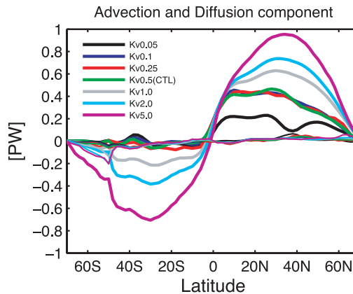
Fig. 9. Meridional oceanic heat transport for all different experiments. Top: total transport including neutral physics. Bottom: advection (heavy lines) and diffusive (light lines) components.
