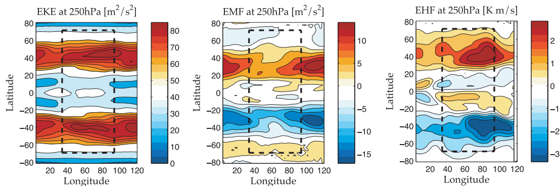
Fig. 13. Eddy Kinetic Energy (EKE), Eddy momentum flux (EMF) and Eddy heat flux (EHF) at 250 hPa for the Atlantic CTL experiment. The dotted squared box represents the ocean basin.
