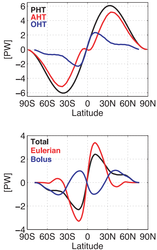
Fig. 17. Meridional heat transports in the Aquaworld experiment. The oceanic (OHT) and atmospheric (AHT) heat transports sum up to give a total, or planetary (PHT), transport of about 6 PW ( 1 \text{ PW} \equiv 10^{15} \text{ W} ) in each hemisphere. The oceanic decomposition into an eulerian and eddy-driven or bolus component is shown in the bottom panel.
