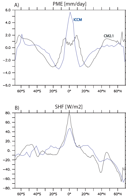
Fig. 4. Precipitation-minus-evaporation (PME, top) and surface total heat flux (SHF, bottom) comparison between the Atlantic ICCM model (blue line) and the CM 2.1 (black line) over the Atlantic Ocean.
