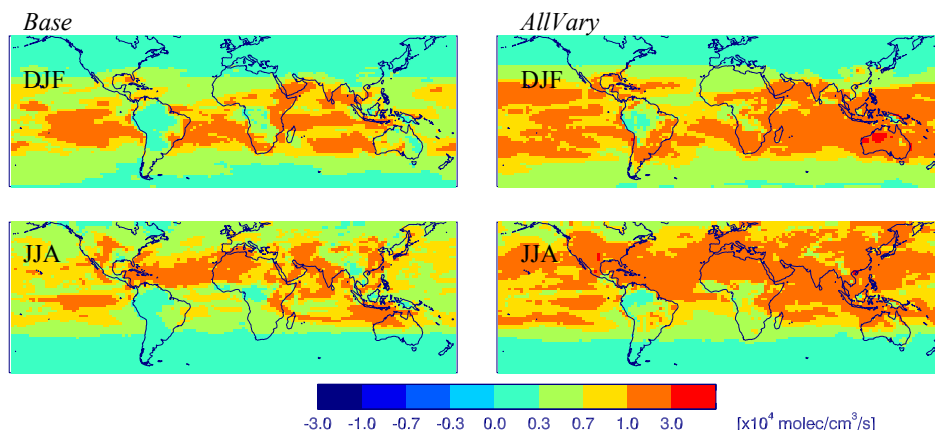
Figure 19. Seasonal mean (1988–2007) standard deviation of tropospheric methane loss rates ( \times 10^4 molecules \text{cm}^{-3} \text{s}^{-1} ) from the Base (left column) and AllVary (right column) scenarios.
