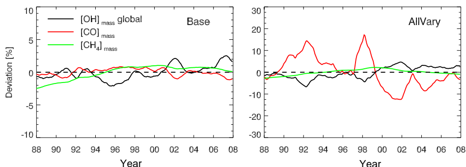
Figure 14. Deviations of tropospheric, mass-weighted OH, CO, and methane (12-month running mean) from the Base (left) and AllVary (right) scenarios. Note the different scales of the y axes.
