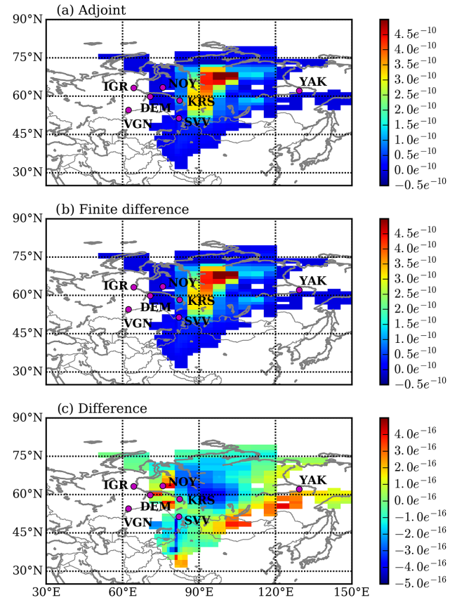
Figure 7. Comparison of sensitivities of \text{CO}_2 concentrations ( \text{ppm} (\mu\text{mol m}^{-2} \text{s}^{-1})^{-1} ) for test 1: (a) sensitivity calculated considering only the Eulerian adjoint model at a resolution of 2.5^\circ , (b) the same sensitivity calculated directly from NIES forward runs using the one-sided numerical finite difference method with perturbations of \varepsilon , and (c) the relative difference between derived adjoint and the numerical finite difference gradients. Magenta dots with labels depict the locations and names of the Siberian observation towers.
