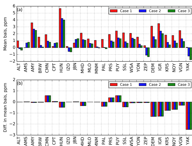
Figure 4. (a) Mean bias for the CO 2 concentrations simulated with the coupled model, (b) difference in mean bias due to the application of the Lagrangian component (for positive bias – the most usual case – negative values mean the results of the coupled model are better than those of the Eulerian model alone) at the selected WDCGG and JR-STATION locations for 2009–2010. The definitions of the cases 1–3 are in Table 1.
