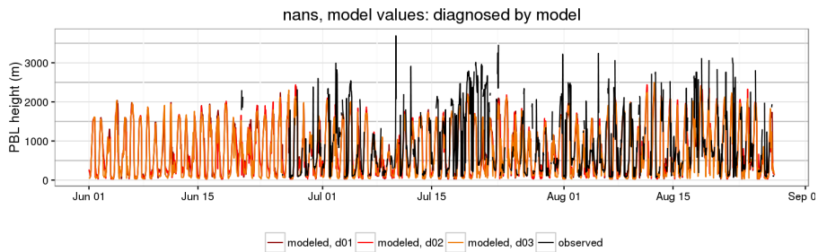
Figure S9. Comparison of modeled PBL height (diagnosed by WRF-Chem) at the Nansenstraße location with the mixing layer height derived from ceilometer observations at Nansenstraße. The results are shown for all three model resolutions (d01 – 15km, d02 – 3km, d03 – 1km).
