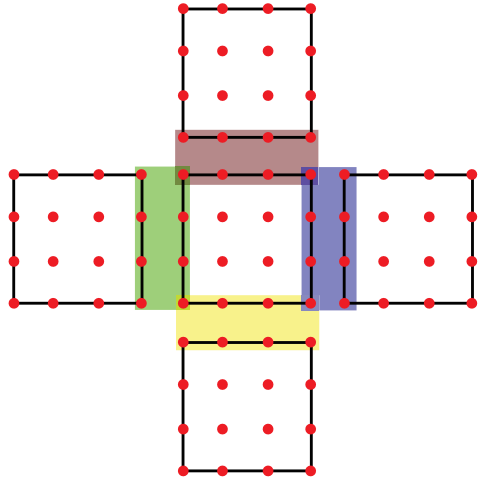
(b) HOMME-DG connectivity.
