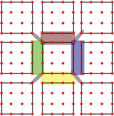
(a) HOMME-SE connectivity.
