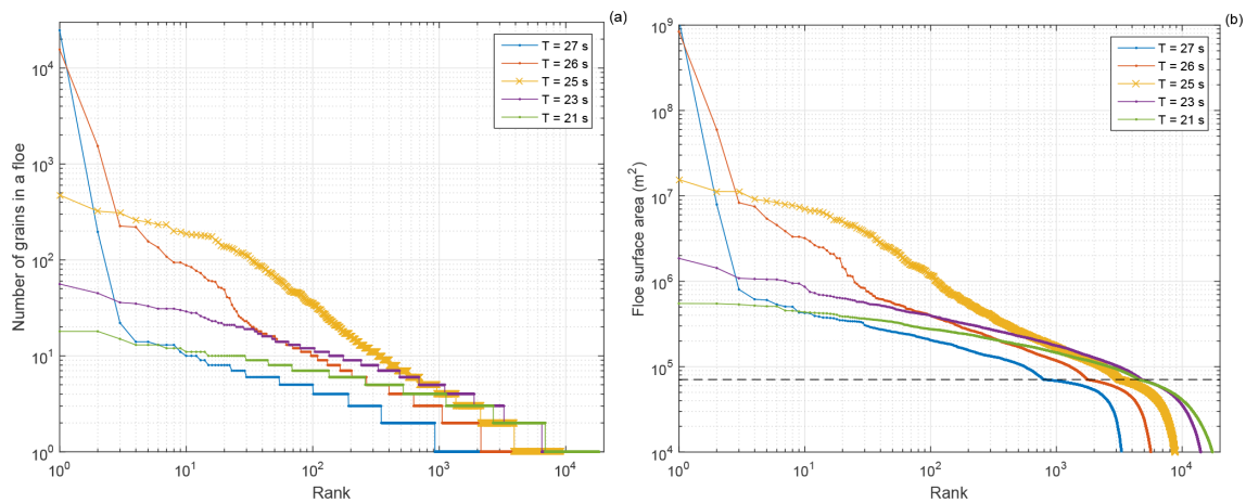
Figure 16. Rank-order statistics of floe sizes ( a : number of grains in a floe; b : floe surface area) obtained in simulations with different wave periods T . The dashed line in ( b ) marks the area of the largest individual grain in the ensemble. Results of the reference run are shown with crosses.
