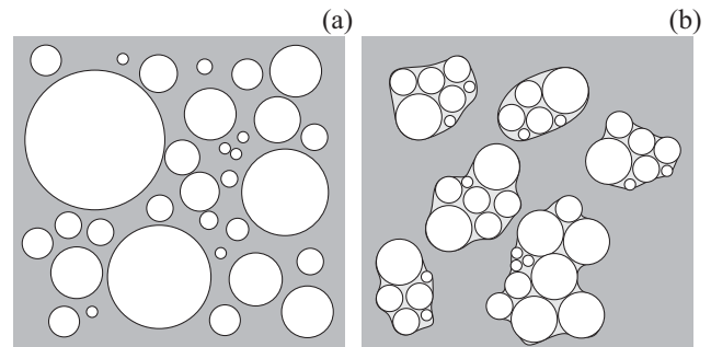
Figure 1. Two approaches to the usage of grains and bonds in DE-Sign: without bonds, when ice floes are identical to grains and the FSD is prescribed (a); with bonds, when ice floes are assemblages of bonded grains and the FSD is obtained as a solution (b).
