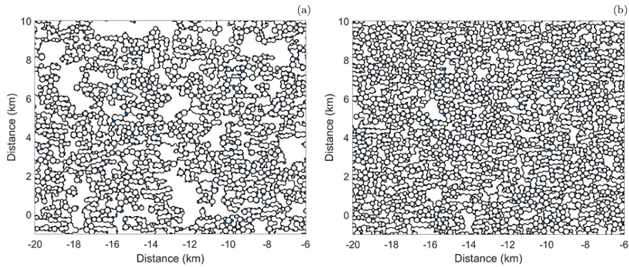
Figure 15. Fragments of the model domain at the end of the reference simulation, with T = 25 s ( a ; wavelength L = 976 m), and a simulation with T = 23 s ( b ; wavelength L = 826 m), showing the pattern of floes. The wave propagation direction is from top to bottom. Note that the whole area of both panels is covered with ice; i.e., the large white spaces are large floes, not open water.
