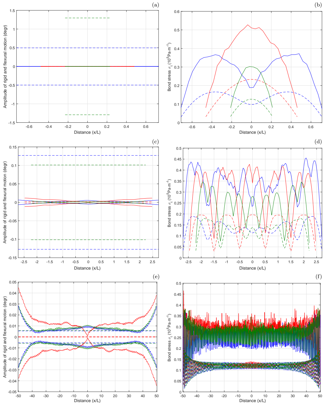
Figure 12. Results of 1-D simulations of sea ice response to waves (without breaking): tilt of the grains ( a , c , e ) and stress acting on bonds ( b , d , f ), for floe lengths equal to (n_0 - \frac{1}{2})L (green), n_0L (red) and (n_0 + \frac{1}{2})L (blue); n_0 = 1 in ( a , b ), n_0 = 5 in ( c , d ), and n_0 = 100 in ( e , f ). In all cases, both ends of the floe could move freely (see text). The distance along the floes is measured relative to the floes' centers. In ( a , c , e ), continuous lines show the range of variability (i.e., the minimum and maximum values recorded during a simulation) of the flexural components of the floe's motion; analogously, the dashed lines show the range of variability of the rigid motion. In ( b , d , f ), the continuous and dashed lines show the maximum and the standard deviation of the stress, respectively. Note different ranges of the vertical axes in the panels. Note that in ( a ), the dashed and continuous red lines cannot be distinguished due to very small values.
