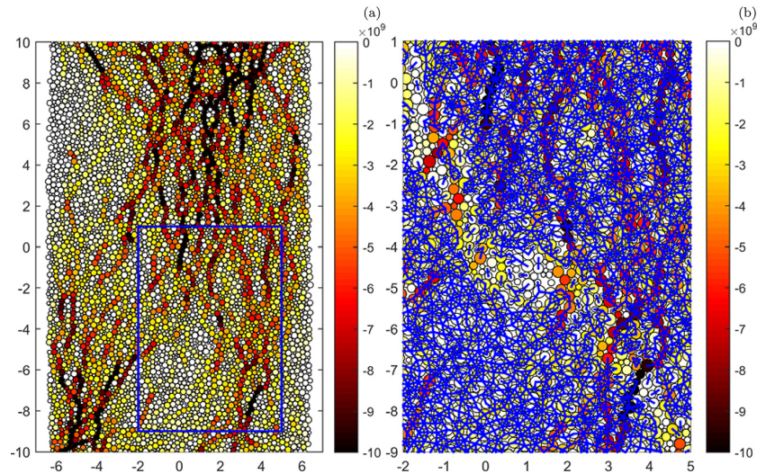
Figure 10. Instantaneous normal stress (color scale; in Pa) acting on individual grains in simulation under uniaxial compressive strain shortly after terminal failure of the material ( t = 600 s; see Figs. 6 and 8). Panel (b) shows a fragment within the rectangle marked in (a), with bonds between grains illustrated with thick blue lines. Reference model settings.
