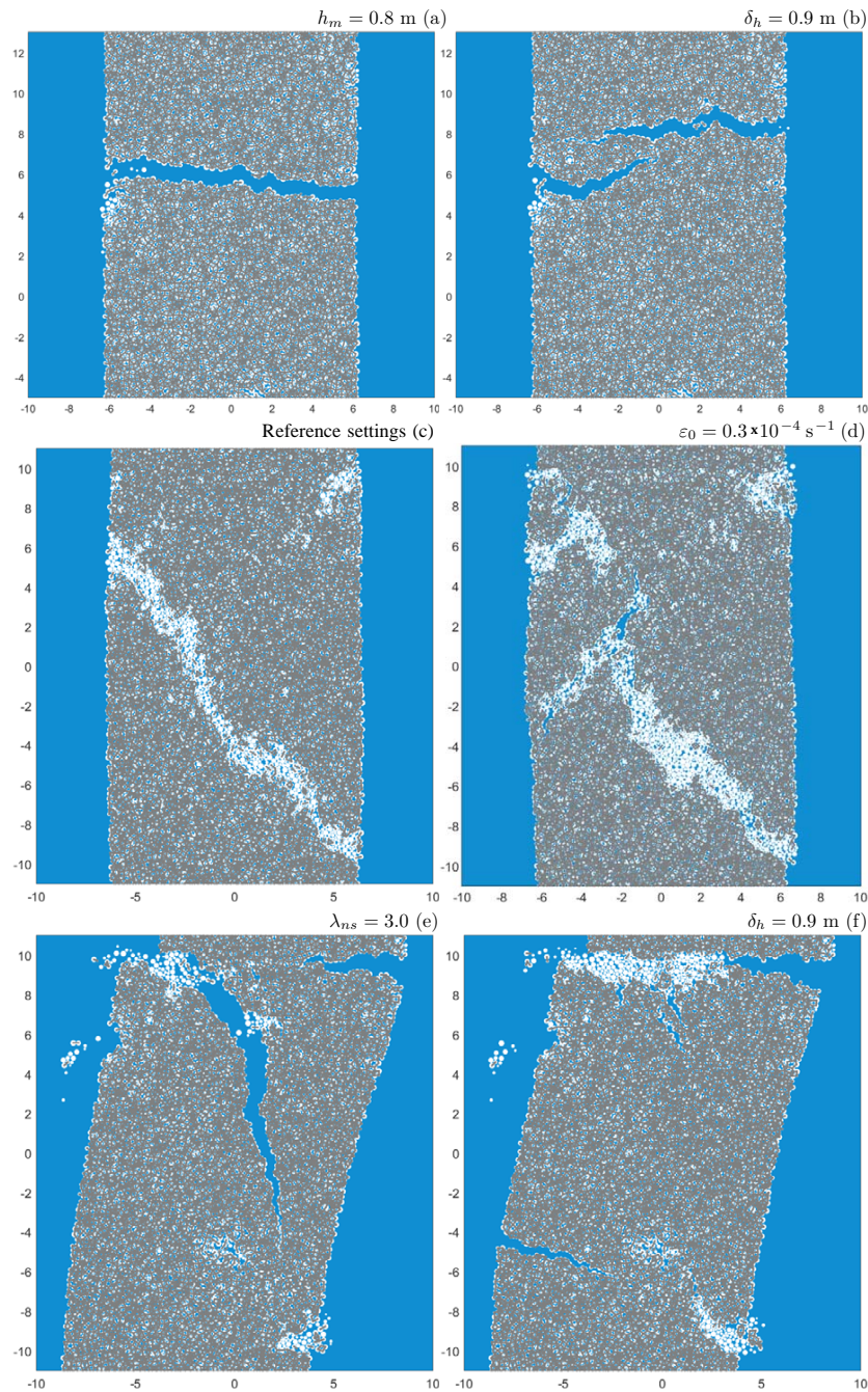
Figure 5. Example damage patterns obtained in simulations of an initially compact sample under uniaxial tensile ( a , b ), uniaxial compressive ( c , d ), and shear ( e , f ) strain. Thick gray lines show the bonds between grains. Model parameters that differed from the reference run are given with each panel. See Figs. S3–S5 for more images.
