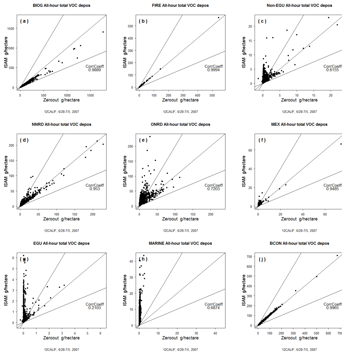
Supp Figure 10. ISAM/V-out scatter plots of all-hour total VOC deposition for each sector. The sectors are: (a) biogenic BIOG, (b) wild fires FIRE, (c) non-electricity generation units NON-EGU, (d) non-road mobile NNRD, (e) on-road mobile ONRD, (f) Mexican point sources MEX, (g) electricity generating units EGU, (h) marine MARINE, and (j) boundary conditions BCON.
