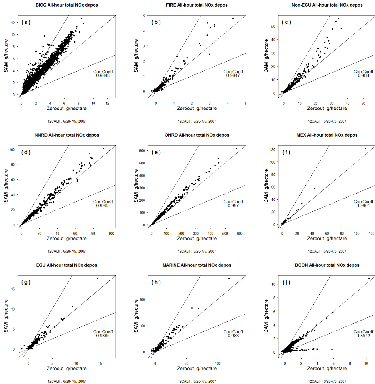
Supp Figure 8. ISAM/N-out scatter plots of all-hour total NOx (NO+NO 2 ) deposition for each sector. The sectors are: (a) biogenic BIOG, (b) wild fires FIRE, (c) non-electricity generation units NON-EGU, (d) non-road mobile NNRD, (e) on-road mobile ONRD, (f) Mexican point sources MEX, (g) electricity generating units EGU, (h) marine MARINE, and (j) boundary conditions BCON.
