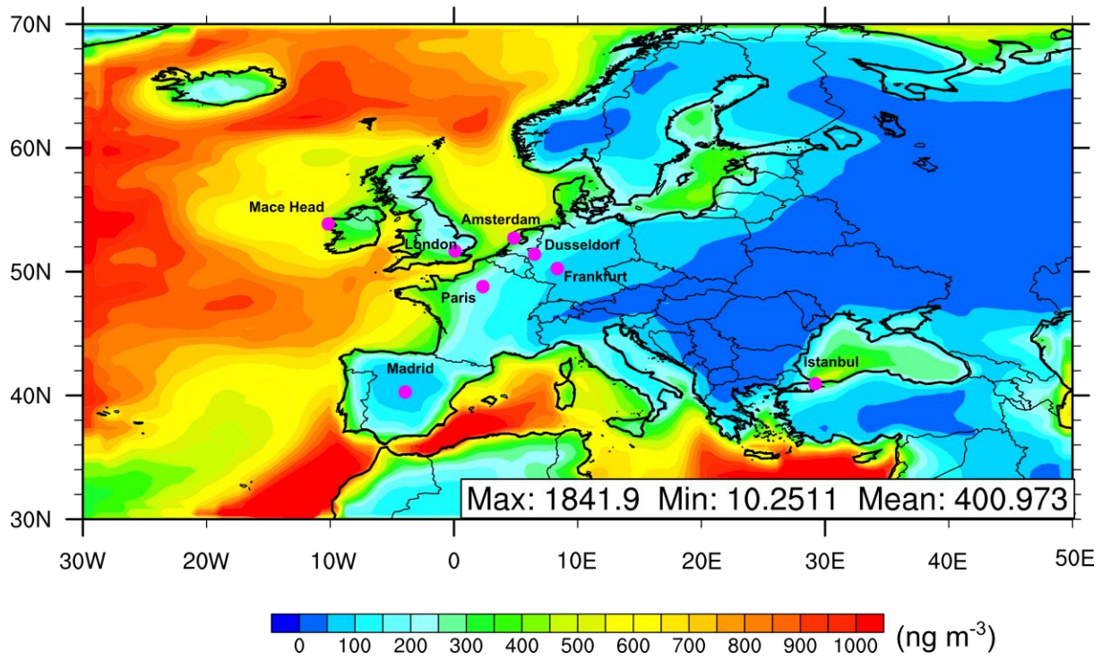
Figure S2. Average surface concentration of submicron sea-salt aerosol for July 2009 in the nested Europe GEOS-Chem domain.
