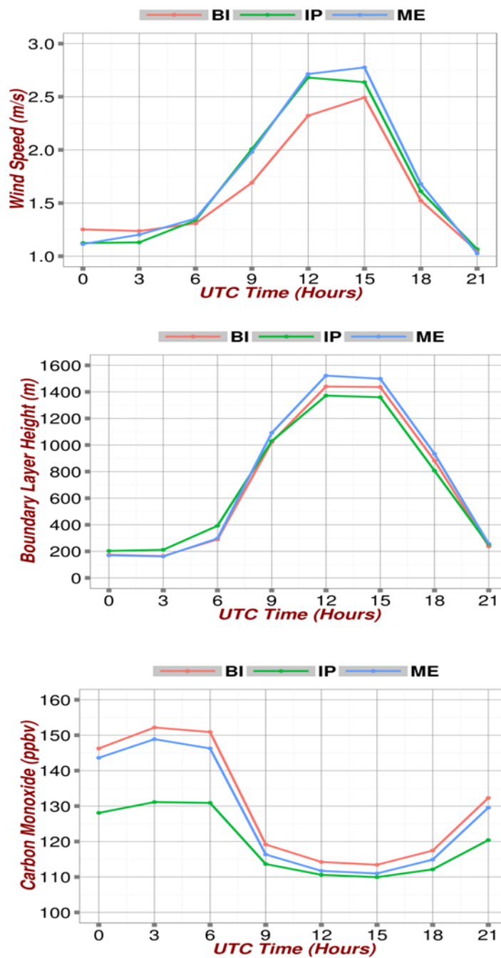
Fig S1 Diurnal meteorological patterns of wind speed (upper panel) and boundary layer height (middle panel) and Carbon monoxide (bottom panel).
