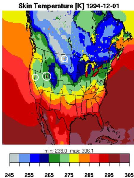
Figure 2. The skin temperature (K) processed from CESM to the 36 km WRF grid using WPS and valid at 00:00 UTC, 1 December 1994. White circles indicate the locations of Pyramid Lake, Great Salt Lake, and Lake Sakakawea, from west to east, respectively.
