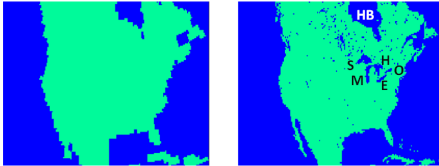
Figure 1. The ocean mask from the 1° CESM data (which is used by WPS to determine the locations of land and water points from CESM), as shown in the area corresponding to a WRF 36 km continental US domain (left), and the 36 km WRF grid's land–water mask (right). Labels are placed to indicate the locations of Lake Superior (“S”), Lake Michigan (“M”), Lake Huron (“H”), Lake Erie (“E”) and Lake Ontario (“O”), as well as Hudson Bay (“HB”).
