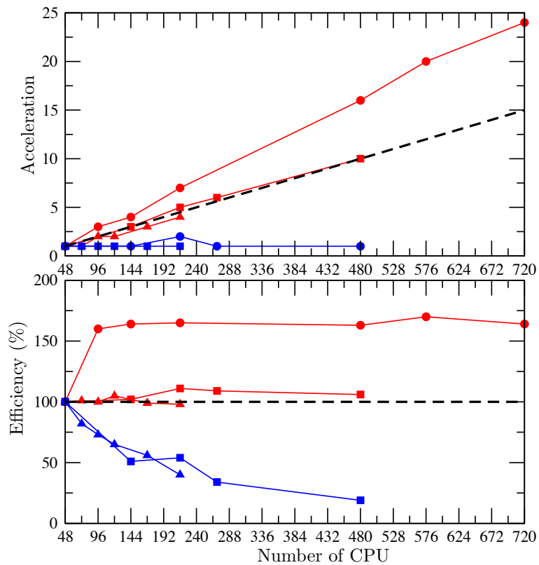
Fig. 3. Acceleration (Up) and efficiency (Bottom) for strong scalability experiments using the block preconditioner for meshes with (red ●) 2.400 \times 10^6 nodes, (red ■) 1.142 \times 10^6 nodes and (red ▲) 0.708 \times 10^6 nodes, and the MUMPS solver for meshes with (blue ■) 1.142 \times 10^6 nodes and (blue ▲) 0.708 \times 10^6 nodes. The dashed line indicates a theoretical efficiency of 100%.
