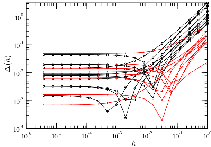
Fig. 6. Ratio \Delta(h) obtained with the Robin (black curves) and Control (red curves) inverse methods for perturbations of the enhancement factor to the viscosity E_\eta(x, y) .
