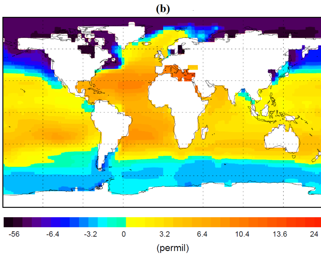
1 2 Figure 1S. The prescribed (a) \delta^{18}\text{O} and (b) \delta\text{D} distribution in ocean surface waters in 3 ECHAM5-wiso.
