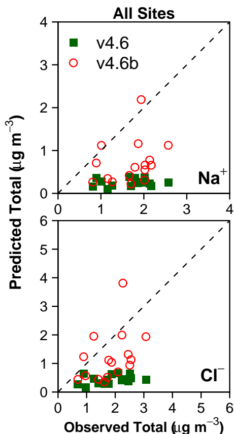
Fig. 3. Modeled total sodium and chloride particle concentrations vs. 23-h impactor observations at three Tampa-area sites for 5 sampling days (6 at Azalea Park) during 2–15 May 2002. “v4.6” indicates CMAQv4.6; “v4.6b” indicates CMAQv4.6b; see Table 1 for version description. For reference, the dashed line represents 1:1 ratio.
