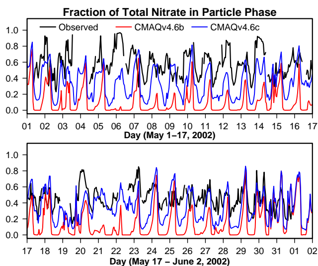
Fig. 6. Time series of observed and modeled fraction of total nitrate in the particle phase [i.e., \text{NO}_3^- / (\text{HNO}_3 + \text{NO}_3^-) ] at the Sydney, FL site from 1 May–2 June 2002. Tick marks represent 00:00 local standard time on each day.
