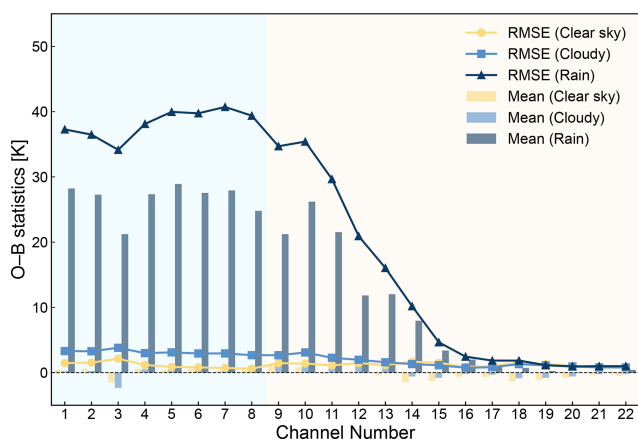
Figure 10. RMSE and mean O–B for the YKW-1 at Yan'an station across all channels from January to June 2025, grouped by clear-sky, cloudy, and rainy conditions.
