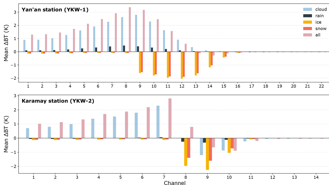
Figure 4. Mean hydrometeor-induced brightness-temperature responses ( \Delta BT ) by channel for YKW-1 at Yan'an and YKW-2 at Karamay. The results are based on ARMS-gb v2.0 simulations driven by 2135 and 2845 hourly cloudy non-precipitating ERA5 profiles, respectively. Bars show the responses to cloud liquid water, rainwater, cloud ice, and snow included separately, together with the combined response when all four species are included. \Delta BT is calculated relative to the corresponding clear-sky simulation.
