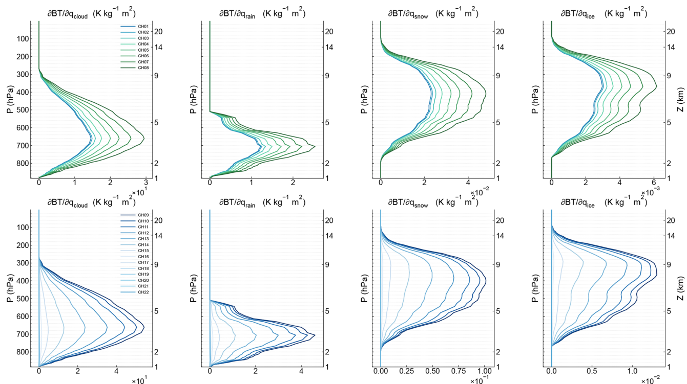
Figure 5. Mean brightness-temperature Jacobians with respect to hydrometeor water paths for YKW-1 at Yan'an under zenith-viewing geometry, averaged over 2135 cloudy non-precipitating hourly ERA5 profiles from January–June 2025. Columns represent cloud liquid water, rainwater, snow, and cloud ice; the upper and lower rows show channels 1–8 and 9–22, respectively.
