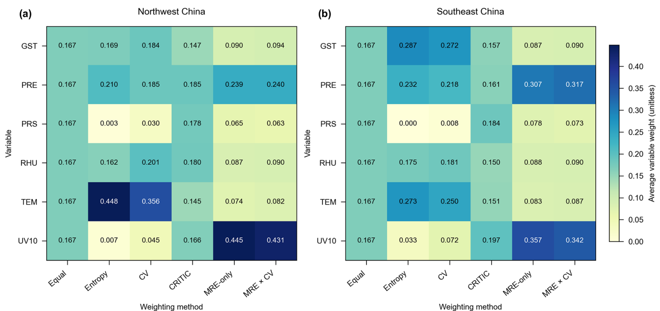
Figure 8. Comparison of average variable weights derived from equal weighting, entropy weighting, coefficient-of-variation weighting, CRITIC weighting, the MRE-only baseline, and the proposed MRE \times CV weighting. Values represent averages across the five physical-process evaluation stages. The MRE-only and proposed weights were calculated from the same candidate set at each stage. (a) Arid region of Northwest China; (b) coastal region of Southeast China. Weights are unitless.
