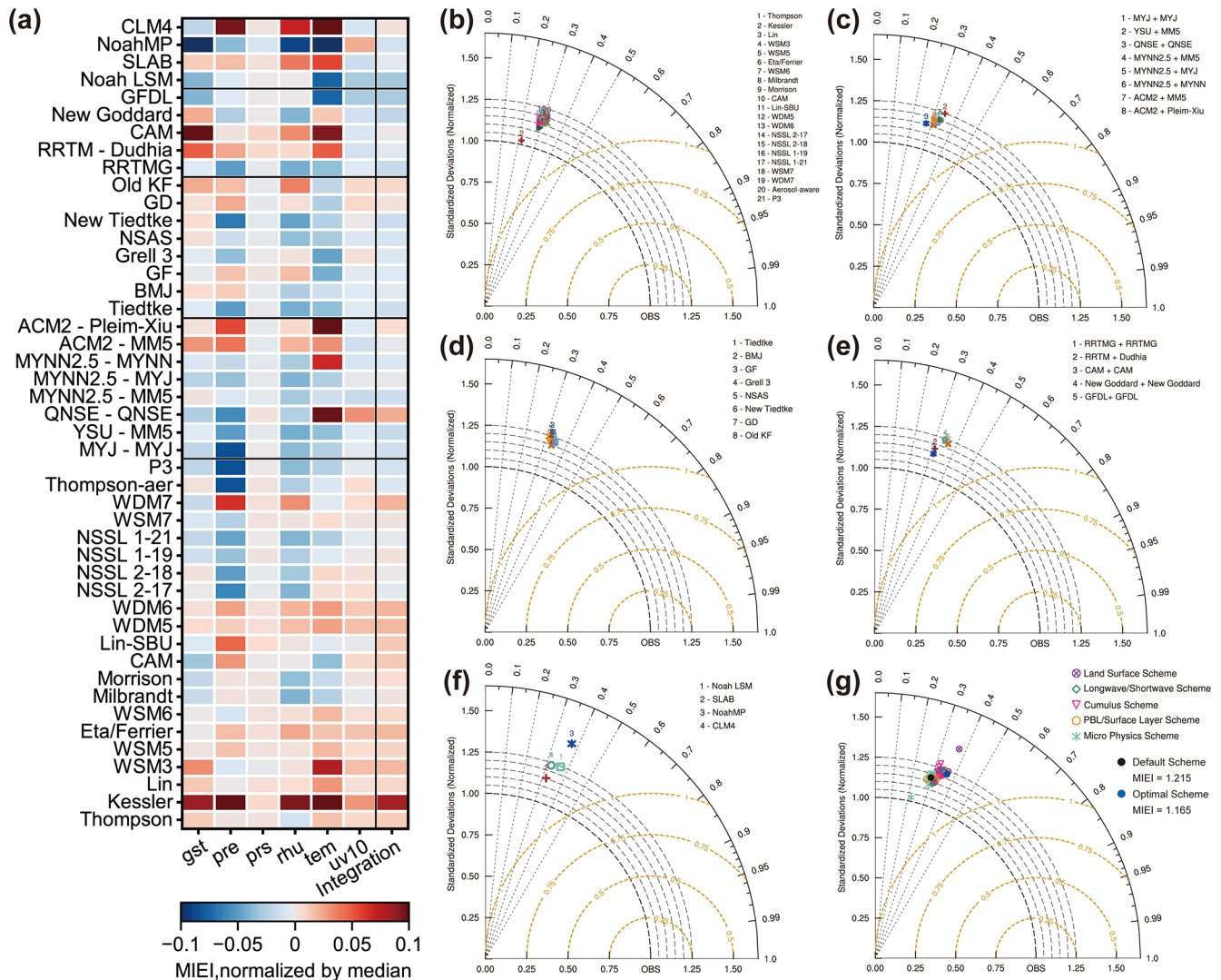
Figure 3. Evaluation results of parameterization schemes in the arid region of Northwest. (a) Median-relative cMIEI, (\text{cMIEI} - C_{\text{med}})/C_{\text{med}} , where C_{\text{med}} is the regional reference median calculated separately for each variable column and the integrated column. This transformation is for visualization only; negative values indicate lower cMIEI. Colors saturate at \pm 0.10 . (b–f) Taylor diagrams of different physical processes. (b) Microphysics, (c) Planetary boundary layer, (d) Cumulus, (e) Radiation, (f) Land surface, and (g) Taylor diagrams of the candidate configurations pooled across all five physical-process stages. All cMIEI and Taylor-diagram statistics were calculated from daily station-level June–August values.
