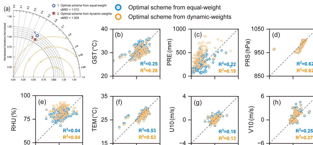
Figure 7. Comparison of simulation results obtained from the optimal parameterization schemes using the proposed \text{MRE} \times \text{CV} weighting and equal weight methods. (a) Taylor plots of the optimal parameterization schemes obtained by different methods. (b–h) Scatter plots of the optimal parameterization schemes obtained via different methods for different meteorological elements. (b) Surface temperature, (c) precipitation, (d) Air pressure, (e) Relative humidity, (f) Air temperature, (g) Zonal wind, (h) Meridional wind. Panel (a) uses Taylor-diagram and cMIEI statistics calculated from daily station-level June–August values; panels (b)–(h) use monthly station summaries only for visual comparison, with monthly means for non-precipitation variables and monthly totals for precipitation.
